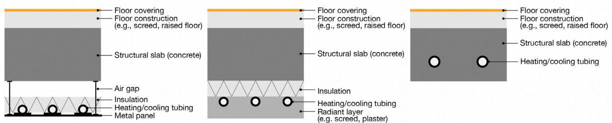
Figure 1: Illustration of radiant panels (left), embedded surface systems (ESS) (center) and thermally activated building systems (TABS) (right)
