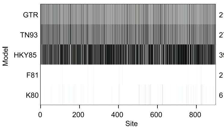
Figure 2. Results from an SDPM2 partition and substitution model averaging analysis of mtDNA from 7 species of primate (data from [22]). (a) The posterior probability distribution of the substitution model given a site. The grid cell at row i and column j represents the posterior probability of model i at site j . The darker the shade, the higher the posterior probability. It appears that this data favours models that accommodate a difference in transition and transversion rates and in nucleotide base frequencies. Of those three models, the simplest version (HKY85) is generally preferred. (b) There are four biological partitions in this data set: the three codon positions and a tRNA region. Conditioned on three rate categories (which has the highest posterior probability), the mean posterior proportion of sites in each category for each biological partition is plotted. The categories with faster rates are closer to the top of the bar. doi:10.1371/journal.pcbi.1003537.g002
