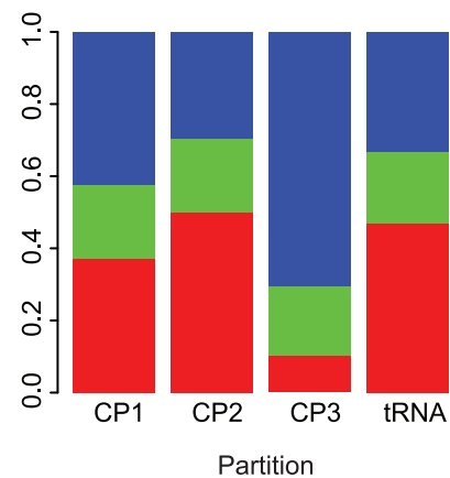
Figure 2. Results from an SDPM2 partition and substitution model averaging analysis of mtDNA from 7 species of primate (data from [22]). (a) The posterior probability distribution of the substitution model given a site. The grid cell at row i and column j represents the posterior probability of model i at site j . The darker the shade, the higher the posterior probability. It appears that this data favours models that accommodate a difference in transition and transversion rates and in nucleotide base frequencies. Of those three models, the simplest version (HKY85) is generally preferred. (b) There are four biological partitions in this data set: the three codon positions and a tRNA region. Conditioned on three rate categories (which has the highest posterior probability), the mean posterior proportion of sites in each category for each biological partition is plotted. The categories with faster rates are closer to the top of the bar. doi:10.1371/journal.pcbi.1003537.g002
