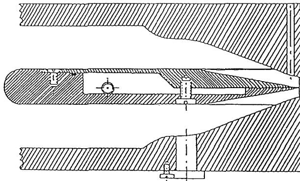
Fig. 1 Two-dimensional air blast atomizers: (a) prefilming atomizer, (b) fixed sheet thickness atomizer (Rizk and Lefebvre, 1980)
