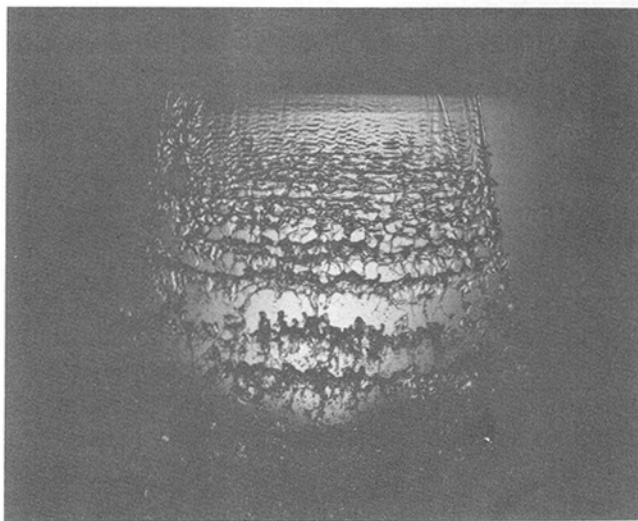
Fig. 7(a) Effect of liquid properties on "cellular breakup": face view, water and ethanol (Case 13)
