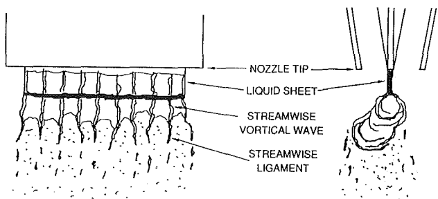
Fig. 3 Schematic of face and side views detailing the structures in the breakup of a liquid sheet for (a) cellular breakup, and (b) stretched streamwise ligament breakup (Stapper and Samuelsen, 1990)
