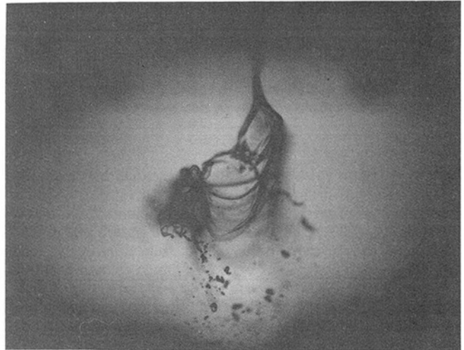
Fig. 5 "Stretched streamwise ligament breakup" (Stapper and Samuelsen, 1990): water sheet at 1 m/s with 20 m/s co-flow air: (a) face view, (b) side view
