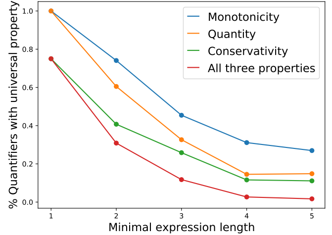
Figure 2: Percentage of universal property per minimal expression length.
