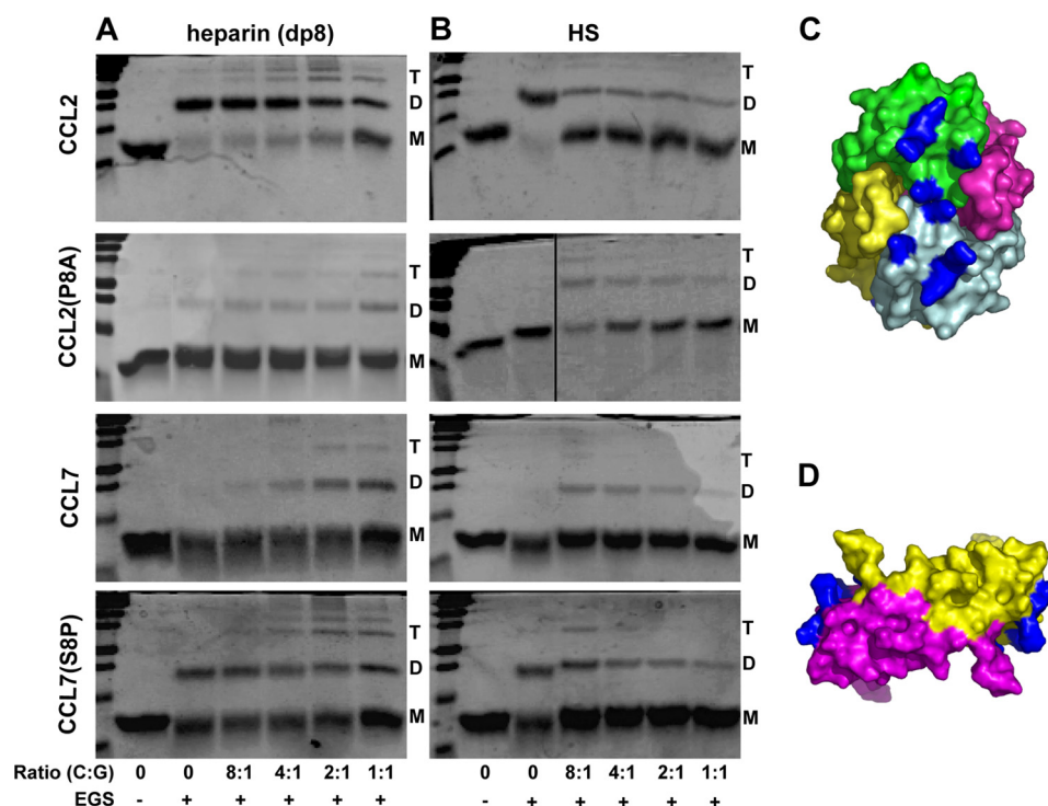
FIGURE 2. Chemical cross-linking of CCL2, CCL2(P8A), CCL7, and CCL7(S8P) with heparin octasaccharide or HS. Chemokine (10 \mu M) was mixed with increasing concentrations of heparin octasaccharide (A) or HS (B) followed by cross-linking with Sulfo-EGS and formation of oligomeric species was evaluated by SDS-PAGE. Tetramer (T), dimer (D), and monomer (M) species are indicated. C and D, structures of CCL2 with known GAG-binding epitopes highlighted in blue illustrate the potential complementarity between heparin and HS with the different oligomeric structures of CCL2. C, the structure of CCL2 shows a continuous linear band of GAG-binding sites (highlighted in blue) in the context of the tetramer (PDB code 1DOL), which is stabilized by binding to highly sulfated heparin chains (11). D, the dimer structure of CCL2 (PDB code 1DOM) with basic GAG-binding patches (highlighted in blue), spatially separated by a relatively charge-neutral area of the dimer structure, is stabilized by HS. HS chains generally consist of unsulfated N -acetylated domains flanked by sulfated domains that may complement the dimer structure (55, 57), in contrast to the more uniformly sulfated heparin, which stabilizes the tetramer structure.
