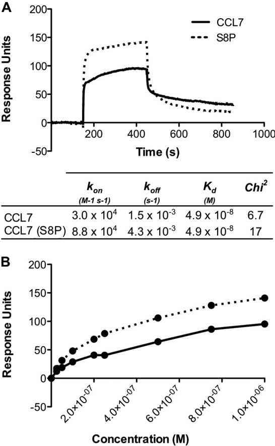
FIGURE 4. The S8P mutation of CCL7 enhances accumulation on HS, whereas affinity is unchanged. A, SPR sensorgram comparing 1 \mu M CCL7 (solid line) and CCL7(S8P) (short dash) on a HS surface and accompanying kinetic analysis from a concentration series ranging from 25 to 1000 nM. B, corresponding steady state curves of CCL7 (solid line) and CCL7(S8P) (short dash) at various concentrations (25–1000 nM) on a HS surface show enhanced accumulation of CCL(S8P) compared with CCL7.
