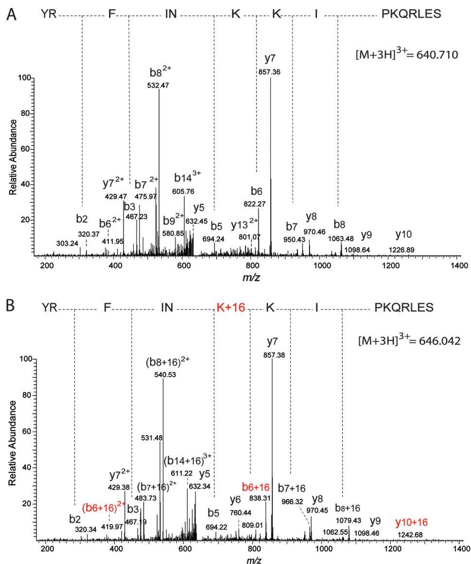
FIGURE 5. MS/MS spectra of the unmodified (A) and modified (B) peptide-(13–27) ( ^{13}\text{YRFINKKIPKQRLES}^{27} ) derived from pepsin digestion of CCL7 following irradiation for 10 ms. The presence of the unmodified b_5 and y_9 ions, and modified b_6 and y_{10} ions (B) shows the modification of this peptide at Lys-18.
