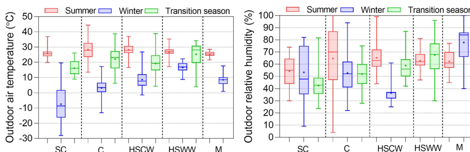
Fig. 9 Outdoor air temperature and relative humidity distributions in different climate zones and seasons.
