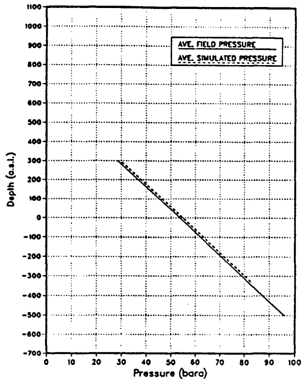
Figure 5. Match between observed and computed pressures for the best model.
