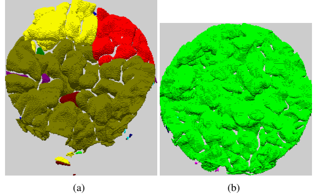
Figure 4. Burning cells within a cylinder of radius 2.5 cm centered in the middle of the data (fuel consumption cut-off: 2.6). (a) SwirlH2 data (t=1500); (b) SwirlH2Fast (t=3000).
