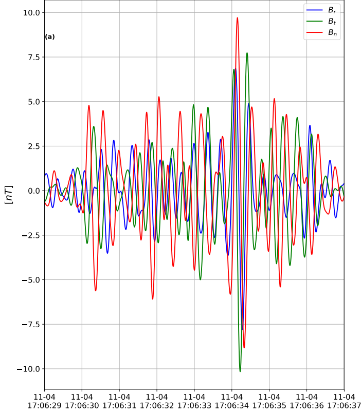
Figure 13. a) Waveforms of magnetic field components in the RTN frame recorded in a close vicinity of the trailing edge of the structure shown in Figure 9. b) Hodograph of the magnetic field in the plane transverse to the wave normal vector.
