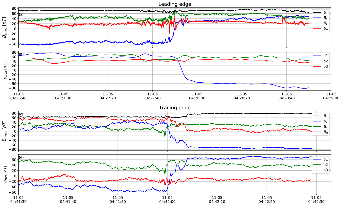
Figure 17. The magnetic field on the structure boundaries: the magnetic field components on the leading edge in the RTN frame (a) and in the MVA frame (b); the magnetic field components on the trailing edge in the RTN frame (c) and in the MVA frame (d).
