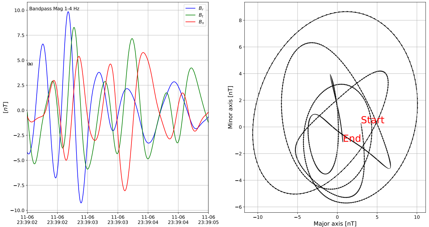
Figure 6. a) Waveforms of the magnetic field fluctuations in the RTN frame filtered in 1-4 Hz frequency band the 3 s time interval on the trailing edge of the structure shown in Figure 2. b) Hodograph of the magnetic field (in the plane transverse to the wave normal) showing close to the circular polarization of the observed wave.
