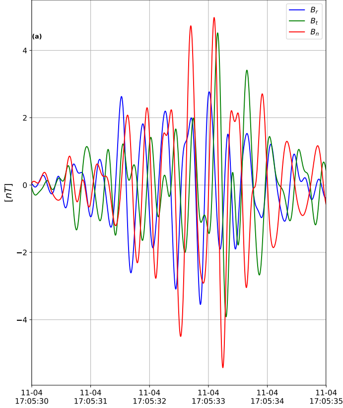
Figure 11. a) Waveforms of magnetic field components in the RTN frame recorded in a close vicinity of the leading edge of the structure shown in Figure 9. b) Hodograph of the magnetic field in the plane transverse to the wave normal vector.
