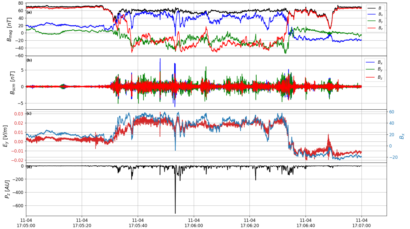
Figure 15. Poynting flux evaluation for compressional structure. a) Magnetic field measurements by MAG instrument during the structure crossing in satellite xyz reference frame, similarly to Figure 7 the data are presented in the satellite reference frame. The components are colored x in blue, y in green and z in red. b) Magnetic field fluctuations registered by SCM instrument, colors are similar to panel a. c) y-component of the electric field registered by FIELDS suite, in red, and x-component of the magnetic field by MAG instrument in blue, the correlation between variations of components is related to the important electric field induced due \mathbf{V} \times \mathbf{B} plasma motion. These fields components are used together with the x-component of the electric field and y-component of the magnetic field for evaluation of the z-component of the Poynting flux. d) z-component of the Poynting flux during time interval including compressional structure crossing. Quite large fluxes directed along the z-axes are registered. It is worth reminding that z axes is quite close to radial direction and the negative flux is directed outward from the Sun.
