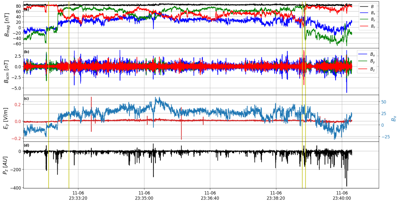
Figure 7. Poynting flux evaluation. a) Magnetic field measurements by MAG instrument during the structure crossing in satellite xyz reference frame. Since there are only two components of the electric field measured on board PSP x and y, for this particular Figure the data is presented in satellite reference frame, contrary to other Figures. The components are colored x in blue, y in green and z in red. b) Magnetic field fluctuations registered by the SCM instrument, colors are similar to panel a. c) y-component of the electric field registered by FIELDS suite, in red, and x-component of the magnetic field by MAG instrument in blue. These fields components are used together with the x-component of the electric field and y-component of the magnetic field for evaluation of the z-component of the Poynting flux. d) z-component of the Poynting flux during time interval including Alfvénic structure crossing. Vertical lines mark the intervals around structure leading and trailing edges.
