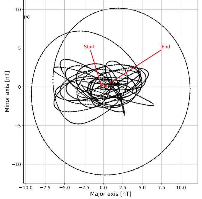
Figure 13. a) Waveforms of magnetic field components in the RTN frame recorded in a close vicinity of the trailing edge of the structure shown in Figure 9. b) Hodograph of the magnetic field in the plane transverse to the wave normal vector.
