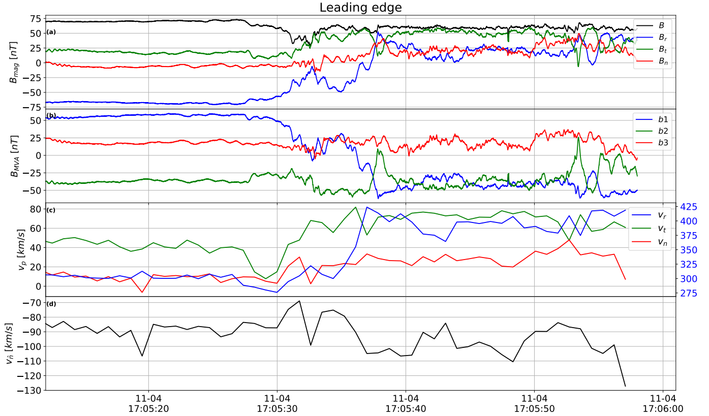
Figure 10. The magnetic field and plasma bulk flow velocity on the leading edge of the compressional structure shown in Figure 9.
