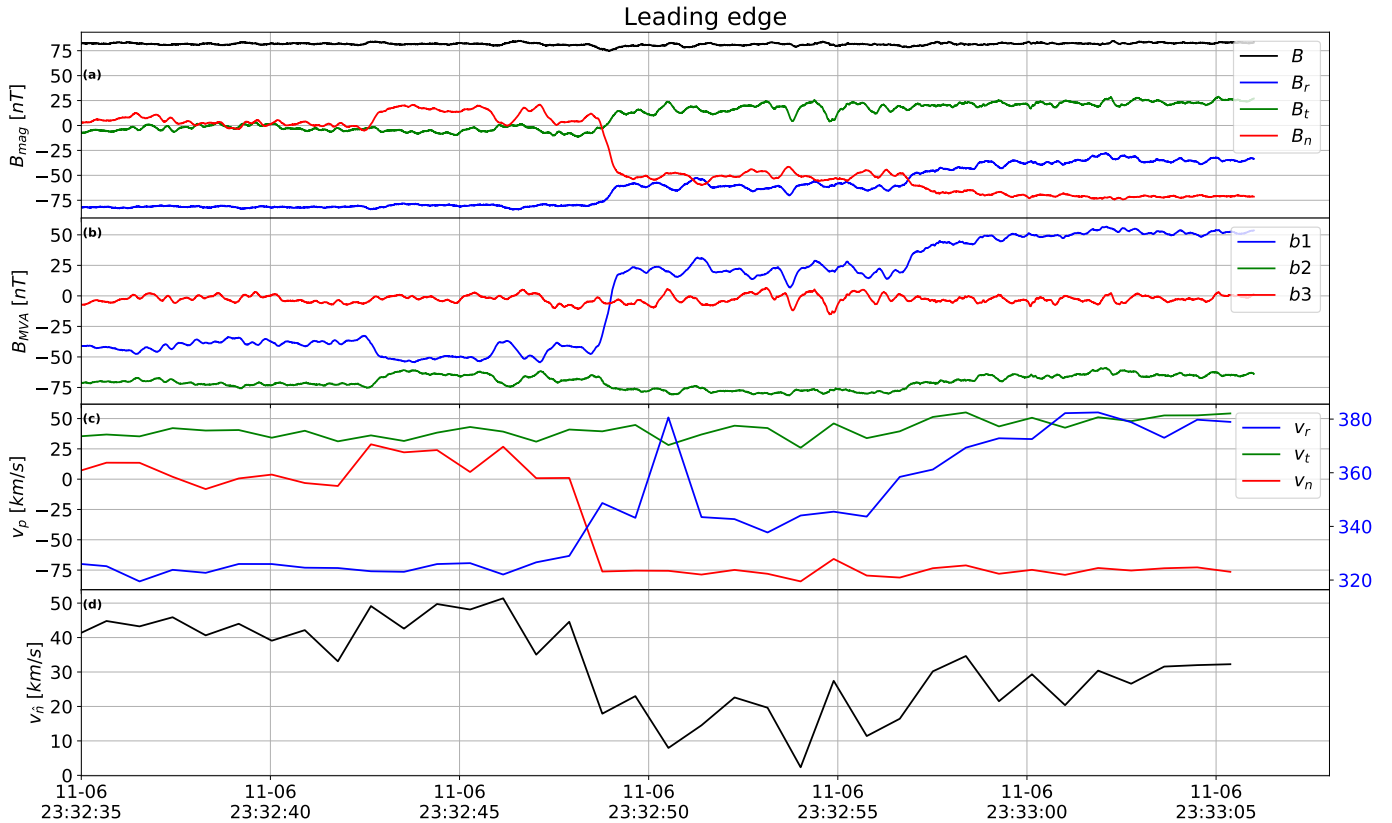
Figure 3. The magnetic field (panel a: in the RTN frame; panel b: in the MVA frame) and plasma bulk velocity (panel c: in the RTN frame and panel d: the normal to the boundary component) on the leading edge the structure shown in Figure 2. The components colors in RTN frame are similar to the ones in Figure 2. In MVA frame the colors are used differently than on other Figures, blue to mark the component corresponding to the largest eigenvalue, i.e. corresponding to largest variation of the field, green to the component corresponding to intermediate value, and red to notify the one related to the smallest eigenvalue, On panel c the largest velocity being strongly different from the others is scaled on the right vertical line.
