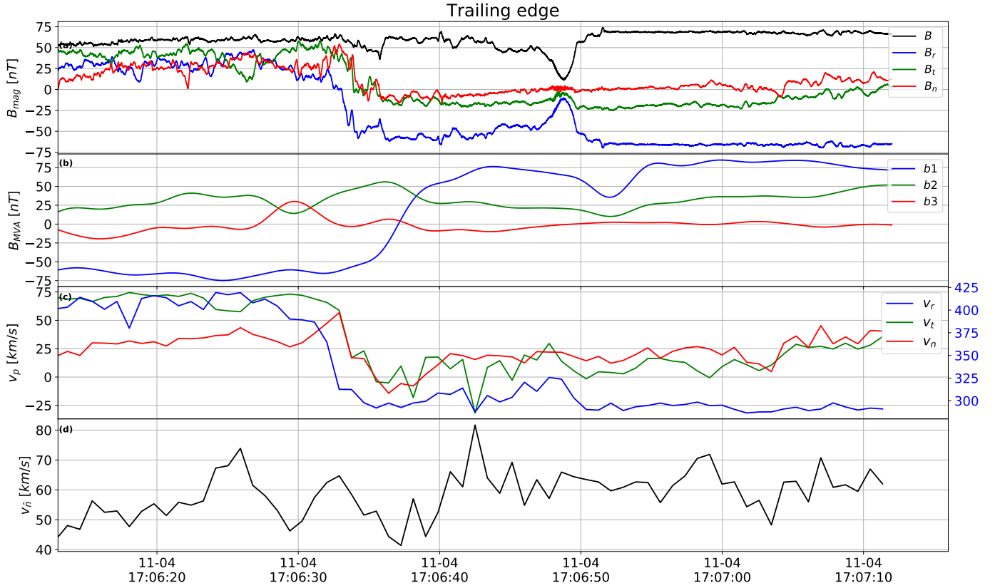
Figure 12. The magnetic field and plasma bulk flow velocity on the trailing edge of the structure shown in Figure 9.
