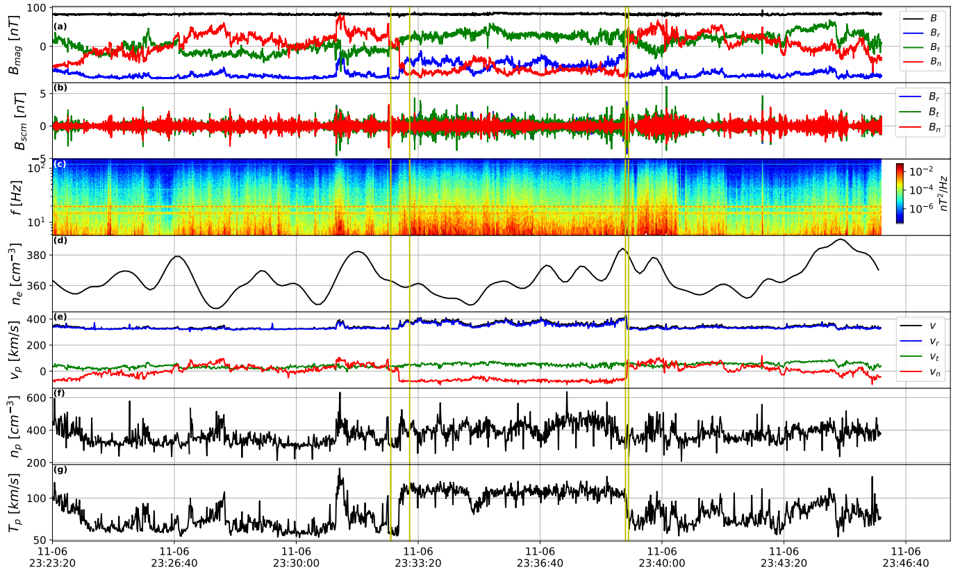
Figure 2. The Alfvénic type magnetic structure detected on November 6, 2018: a) the magnetic field components in the RTN reference frame (the radial component is in blue, the tangential one in green and the normal one in red). The magnetic field magnitude is shown with the black curve. b) magnetic field fluctuations from the SCM instrument (the colors are the same as in panel a. c) the magnetic field fluctuations dynamics spectrum. d) the averaged
