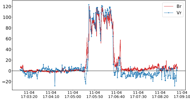
Figure 14. The radial components of the magnetic field (red) and plasma bulk velocity (blue) during crossing of the structure (Figure 9), illustrating close to the linear correlation, i.e. high level of Alfvénicity. The Alfvénic type of perturbations is on the leading edge, however, the change of components around trailing edge is presumably due to the change of plasma parameters across the structure. The y-scale is the same because the respective mean computed over the before encounter data (17:03 to 17:05:26) has been subtracted.
