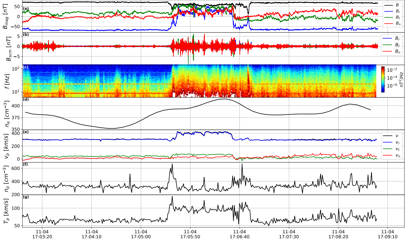
Figure 9. The compressional magnetic structure in the same format as in Figure 2.
