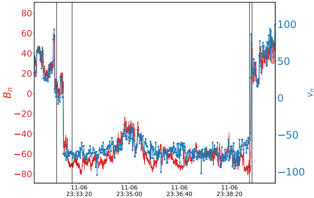
Figure 5. The normal components of the magnetic field (red) and plasma bulk velocity (blue) during crossing of the structure (Figure 2), showing linear correlation. The leading and trailing boundaries are marked by the vertical lines. The variations on the boundaries are synchronous and fit the linear relation.
