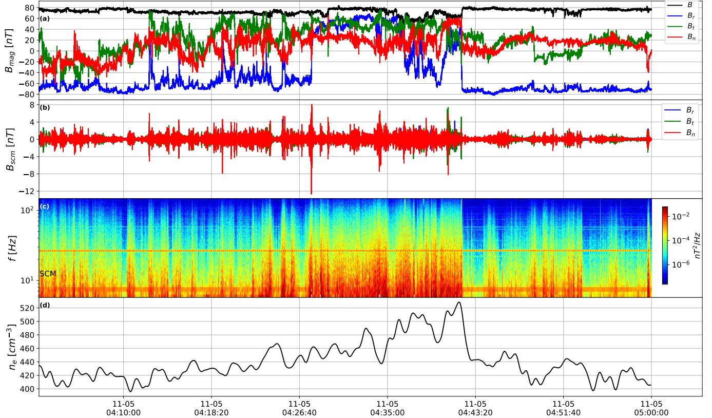
Figure 16. The structure containing the full reversal of the radial component of the magnetic field in the same format as in Figure 2
