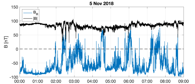
Figure 1. Magnitude (in black) and the radial component (in blue) of the magnetic field recorded on November 5, 2018 from 00:00 to 09:00 UT. Switchbacks show up as sudden increases in the radial component.
