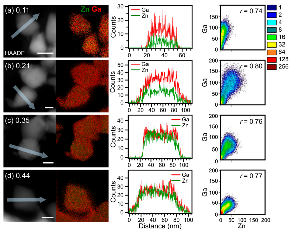
Figure 6. Left column: HAADF-STEM images and EDS elemental maps of (\text{Ga}_{1-x}\text{Zn}_x)(\text{N}_{1-x}\text{O}_x) NCs prepared at 800 °C with ensemble x values of (a) 0.11, (b) 0.21, (c) 0.35 and (d) 0.44. Scale bars are 30 nm. Middle column: EDS line profiles of Zn and Ga taken across an oxynitride particle indicated by arrow for the direction of the profile. Right column: Colocation analyses of the distribution of Zn in relation to Ga for (\text{Ga}_{1-x}\text{Zn}_x)(\text{N}_{1-x}\text{O}_x) NCs. Analyses contain scatter plots of the respective element intensities at each pixel within the single NC area. The resulting Pearson's r is displayed in the top right corner of the scatter plot.
