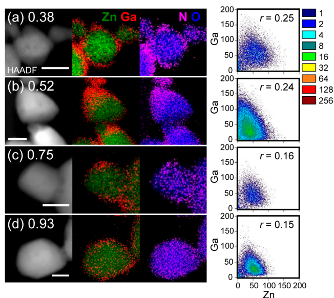
Figure 3. Left column: HAADF-STEM images and EDS elemental maps of (\text{Ga}_{1-x}\text{Zn}_x)(\text{N}_{1-x}\text{O}_x) NCs synthesized at 650^\circ\text{C} with varying ensemble compositions x of (a) 0.38, (b) 0.52, (c) 0.75 and (d) 0.93. The map shows the overlays of two elements, Zn/Ga and N/O. Scale bars are 15 nm. Right column: Colocation analyses of the distribution of Zn in relation to Ga for each (\text{Ga}_{1-x}\text{Zn}_x)(\text{N}_{1-x}\text{O}_x) NC shown on the left. Analyses contain scatter plots of the respective element intensities at each pixel within the single NC area. The resulting Pearson's r value is displayed in the top right corner of the scatter plot.
