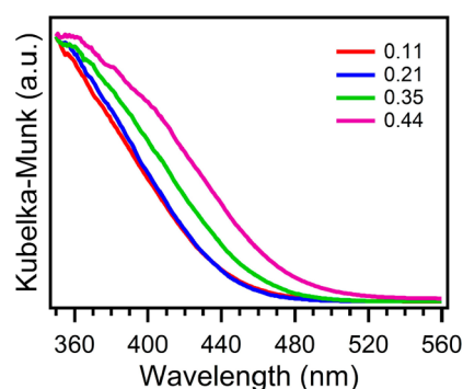
Figure 7. Kubelka–Munk transformed diffuse reflectance spectra of (\text{Ga}_{1-x}\text{Zn}_x)(\text{N}_{1-x}\text{O}_x) NCs synthesized at 800 °C with different compositions ( x = 0.11, 0.21, 0.35 and 0.44 ). The spectra are normalized at 350 nm.
