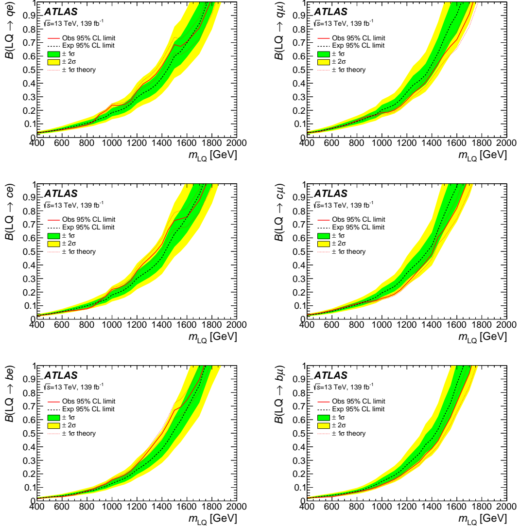
Figure 9: The observed and expected limits on the leptoquark branching ratio \mathcal{B} into a quark and an electron or a muon at 95% CL, shown as a function of m_{\text{LQ}} for the different leptoquark channels. The green and yellow bands show the \pm 1\sigma and \pm 2\sigma ranges of the expected limit. The error band on the observed curve represents the uncertainty in the theoretical cross-section from PDFs, renormalisation and factorisation scales, and the strong coupling constant \alpha_s .
