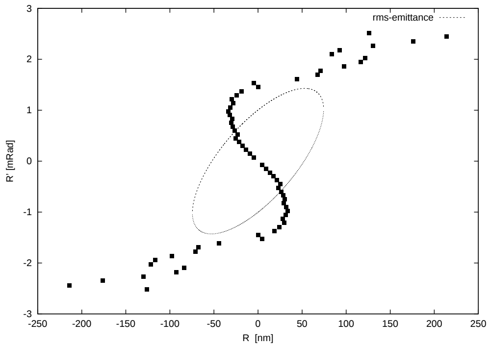
Figure 6. Emittance plot.
