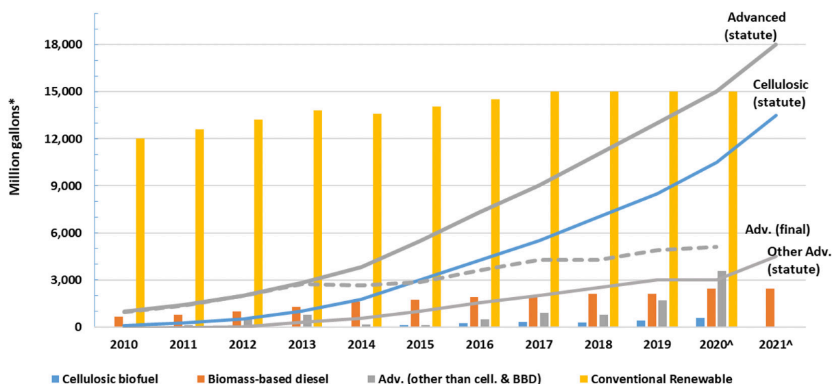
Figure 1. RFS Volume Standards: implemented (columns) and statutory levels (lines). *Gallons for biomass-based diesel (BBD); ethanol-equivalent gallons for other mandates. "Adv. (other than cell. & BBD)" and "Other Adv. (statute)" refer to residual advanced fuel after adjusting for ethanol-equivalent gallons covered through the cellulosic and biomass-based diesel mandates, with the statutory line indicating the statutory minimum of 1 billion gallons. a Calculated before annual volumes finalized, using the statutory minimum for BBD. Data source: (Bracmort 2020) 1
