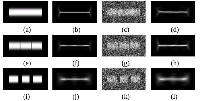
Fig. 6. Performance of the iterative voting method with added noise at SNR = 0 and perceptual boundaries: (a-d) signal delineation in noise free and noisy synthetic object; (e-h) signal delineation in an object (without and with added noise) with small perceptual gaps; and (i-l) signal delineation in an object (without and with added noise) with large perceptual gaps.
