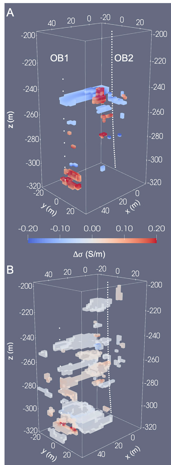
FIGURE 12 | (A): Inversion of CaMI.FRS field data with variable parameter bounds. The inversion is initialized with the layered starting model ( M^{1D} ) obtained from 1D inversion (Figure 9). Shown are deviations \Delta\sigma_{var} = M_{var}^{3D} - M^{1D} where M_{var}^{3D} is the final model update. Only deviations |\Delta\sigma| > 0.075 S/m are visualized, where blue and red regions indicate positive and negative deviations. (Continued)
