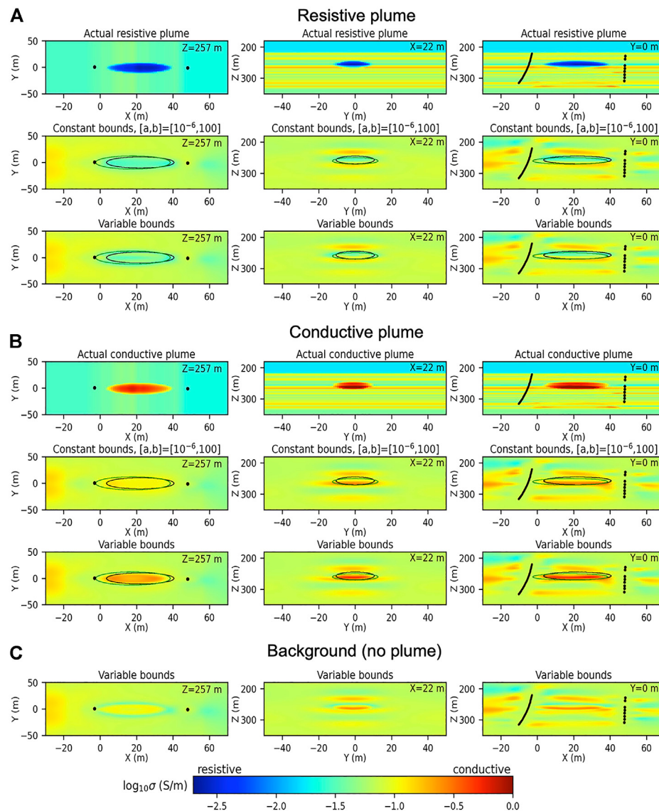
FIGURE 5 | (A): Plume imaging for CaMIFRS. Comparative inversions for an electrically resistive plume model. The upper, middle, and lower plot rows show, respectively, true model, inversion result using constant bounds, and inversion result using spatially variable bounds. (B): Comparative inversions for an electrically conductive plume model. The upper, middle, and lower plot rows show, respectively, true model, inversion result using constant bounds, and inversion result using spatially variable bounds. The corresponding variable lower and upper parameter bounds are shown by Figure 4 . Elliptical contour lines in the images outline true (black) and assumed (green) plume boundaries. Assumed boundaries pertain to the ellipsoidal region defining the variable lower and upper parameter bounds. (C): Inversion of data set created from the background model using the variable bounds.
