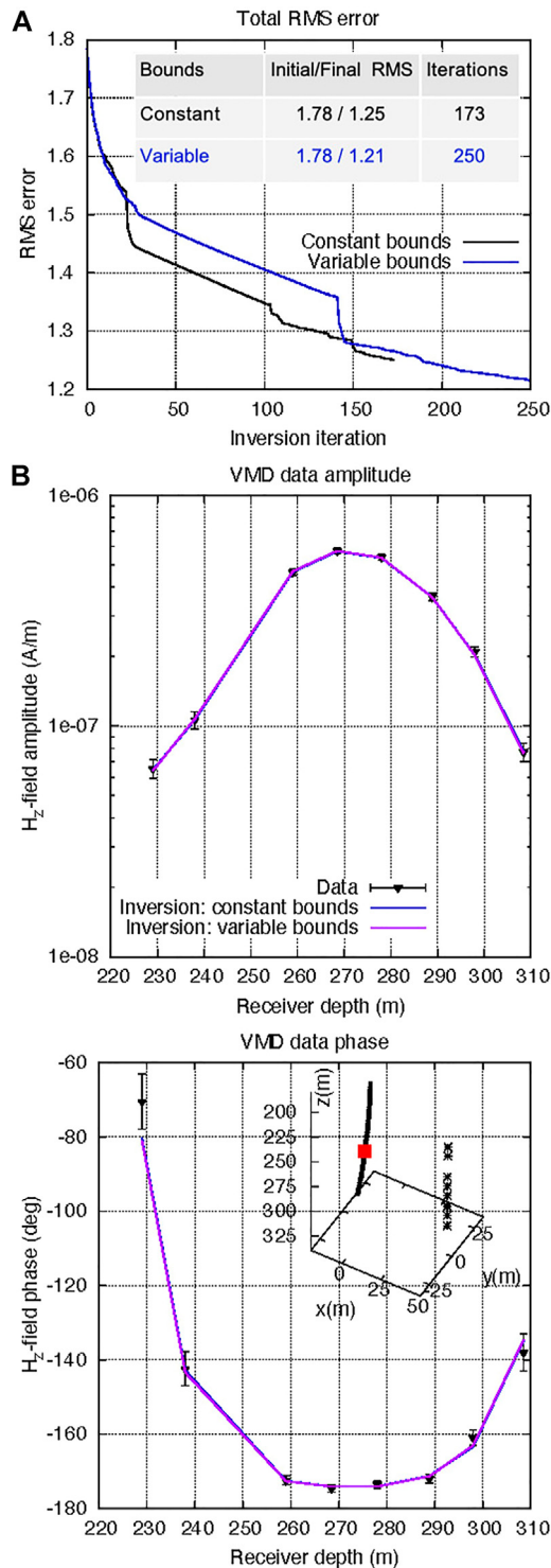
FIGURE 11 | (A): Total RMS fitting error for CaMI.FRS field data inversion. (B): Data (symbols) and fits for inversions with constant bounds (blue lines) and variable bounds (purple lines). Real and imaginary vertical-magnetic fields are converted into amplitude and phase. The exemplified fits correspond to one transmitter-receiver traverse with the source located at z = 270 m (marked by red symbol).
