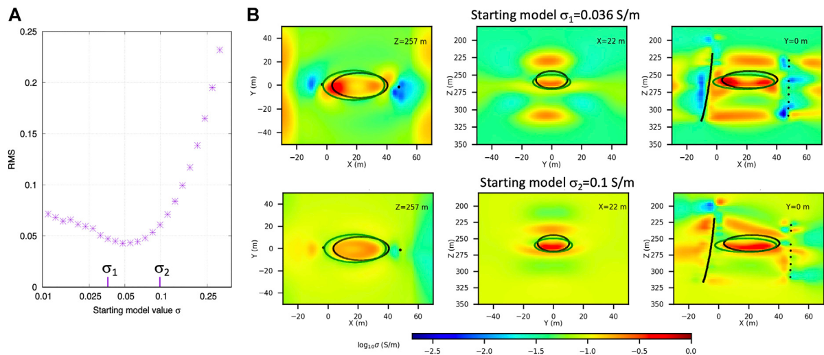
FIGURE 8 | (A): Multiple inversion realizations for the conductive ellipsoidal anomaly (true model shown by Figure 5B , first row) using a range of homogeneous starting model values. The RMS error quantifies the difference between the true model and each inversion result. (B): Model reproductions exemplified for two starting-model values, \sigma_1 = 0.036 S/m and \sigma_2 = 0.1 S/m.
