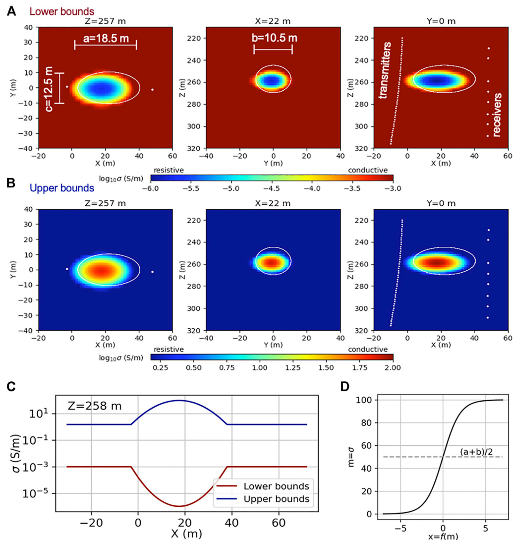
FIGURE 4 | (A): Plume imaging for CaMI-FRS. Spatially variable lower and upper model parameter bounds constrain inversions for an ellipsoidal \text{CO}_2 plume. Variable bounds occur over an ellipsoid that is different in shape and center coordinates to the true plume, the latter indicated by white contours and the semiaxes lengths ( a, b, c ). Crosswell instrument locations are projected. Lower parameter bounds span the electrical-conductivity range from 10^{-6} to 10^{-3} S/m. (B): Upper bounds range from 1.5 to 100 S/m. (C): Lower and upper bounds are paired such that constraints open up when traversing the ellipsoidal target region, here shown for the x -axis at (y, z) = (0, 258) m. (D): The logarithmic transformation function of Eq. 4 is exemplified for the bound interval [a, b] = [10^{-6}, 100] .
