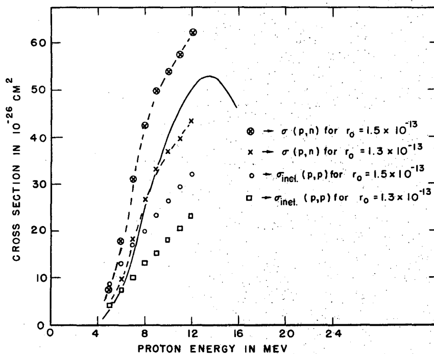
COMPARISON OF THE MEASURED (p,n) CROSS-SECTION ON \text{Cu}^{63} WITH THEORETICAL VALUES, CALCULATED ON THE BASIS OF STATISTICAL THEORY. THE SOLID LINE IS THE EXPERIMENTAL CROSS SECTION CURVE.
