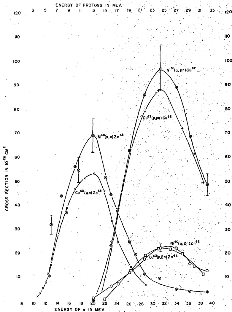
CROSS SECTIONS FOR (p,n), (p,2n), (p,pn) REACTIONS ON \text{Cu}^{63} AND FOR ( \alpha ,n), ( \alpha ,2n), ( \alpha ,pn) REACTIONS ON \text{Ni}^{60} PLOTTED TOGETHER. THE SCALE OF E_p IS DISPLACED BY 7 MEV. WITH RESPECT TO THE SCALE OF E_\alpha . MU 309
