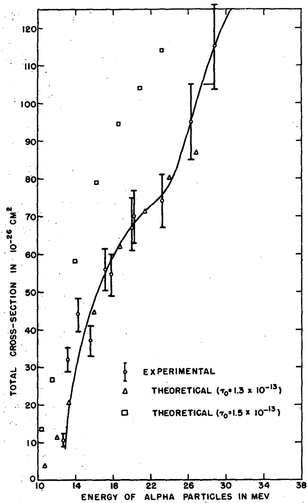
TOTAL CROSS-SECTION WHICH IS THE SUM OF (p,n), (p,2n) (p,pn) CROSS-SECTIONS ON \text{Cu}^{63} AS DETERMINED EXPERIMENTALLY IS COMPARED WITH THEORETICAL \sigma_p WHICH IS THE CROSS-SECTION FOR THE ABSORPTION OF AN \alpha -PARTICLE BY \text{Ni}^{60} NUCLEUS. MV 295
