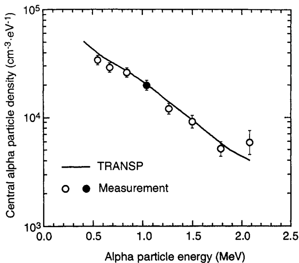
FIG. 4. Alpha particle energy distribution at the centre of a DT plasma 0.2 s after the end of the NBI. The measurements are normalized to the TRANSP calculation at the solid point.
