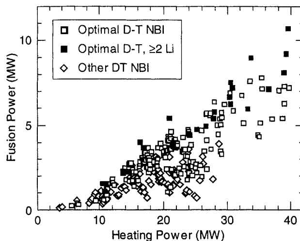
FIG. 2. Dependence of the peak DT fusion power output on the total heating power. The data are for supershots with at least one NBI source injecting pure tritium. Shots with nearly optimal tritium fraction, 0.4 < P_{T-NBI}/P_{NBI} < 0.8 , and shots with two or more lithium pellets before NBI are distinguished.
