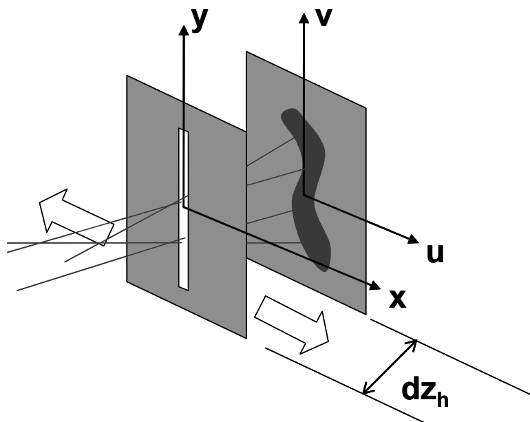
Fig 4. Schematic of the optical slit scanner. The beam ions passing through the first slit produce an image on the scintillator that provides information on their transverse velocity. The technique for converting the information in the scintillator plane ( u, v ) to beam properties at the slit plane ( x, y ) is described in Ref. 6.
