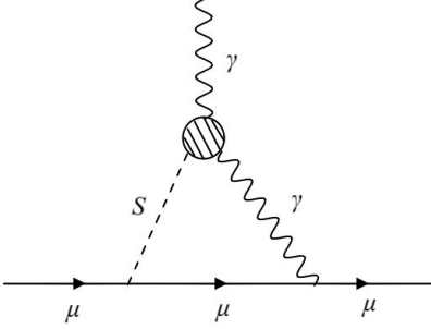
FIG. 1: Contribution of the effective S\gamma\gamma coupling to (g-2)_\mu .
