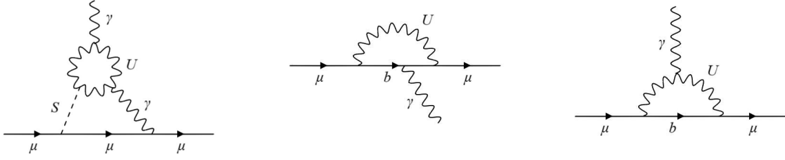
FIG. 4: U leptoquark contributions to (g - 2)_\mu . Left: Two-loop Barr-Zee diagram involving also the dark Higgs boson S . Center and right: One-loop diagrams that are independent of the dark Higgs boson.
