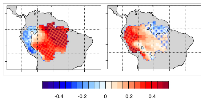
Fig. 5. Linear trends in number of months per year experiencing drought or unusual wetness, 1950–2099. (Left) Months per year experiencing SPI < -2 and (Right) months per year experiencing SPI > 2 . Shown are the mean of results from 35 CMIP5 models. The black line denotes zero trend; i.e., it separates regions of increasing and decreasing drought frequency. Hatching (dots) indicate regions where >2/3 of models have a positive (negative) trend. Units are months per year per century.
