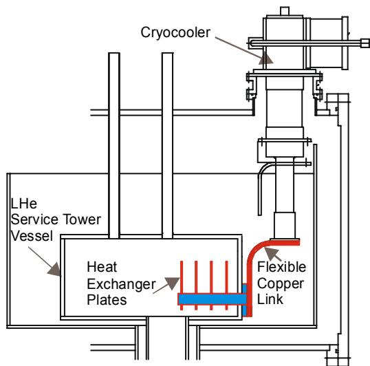
Figure 4 Original Heat Exchanger Design
