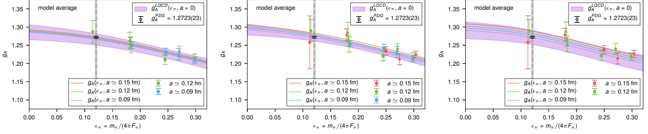
Supplemental Data Figure 5 | Sensitivity to cutting lattice spacings. We plot the resulting model average analysis when either the coarsest or finest ensembles are cut from those considered, with the full data set in the middle for comparison. Uncertainties are one s.e.m.
