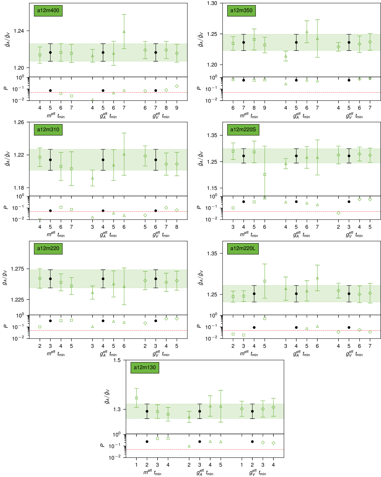
Supplemental Data Figure 17 | Correlator fit t_{\min} stability study II. Analogous to Extended Data Fig. 1e and Supplemental Fig. 16 for the remaining ensembles. Uncertainties are one s.e.m.
