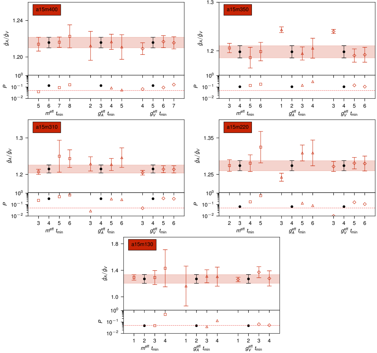
Supplemental Data Figure 16 | Correlator fit t_{\min} stability study I. Analogous to Extended Data Fig. 1e. Solid circles accompanied by shaded bands are the preferred simultaneous fits. Varying fit regions for the two-point correlator ( \square ), and axial ( \triangle ), and vector ( \diamond ) effective derivatives are presented. Corresponding P -values are presented, with the dashed red line at p = 0.05 discriminating statistical significance of the fit results. Uncertainties are one s.e.m.
