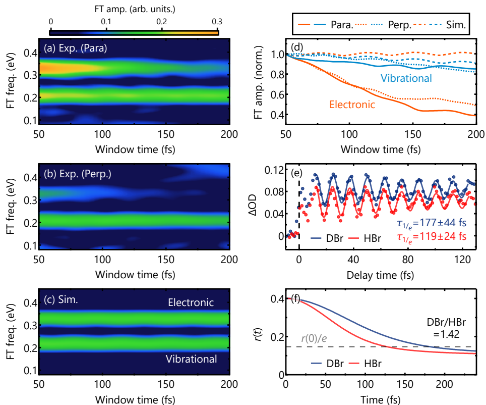
FIG. 5. (a-c) Time-window Fourier transformation analysis of the (a) experimental parallel measurement, (b) experimental perpendicular measurements, and (c) simulated results. Time evolution of the oscillation amplitude from the electronic and vibrational coherences are extracted. (d) Normalized signal amplitude for the electronic quantum beats (orange) and vibrational quantum beats (blue). The electronic quantum beats in the parallel (solid curve) and perpendicular (dotted curve) measurements exhibit a partial decrease, whereas the simulated result (dashed curve) maintains a constant amplitude. (e) A comparison of the electronic quantum beats between the DBr (blue) and HBr (red) results. The dots show the experimental absorption signals at 66.7 eV, and the solid curves show the fitting with a cosine function and an exponential decay. The fitted decay times ( \tau_{1/e} ) are 177 \pm 44 fs for DBr, and 119 \pm 24 fs for HBr, which yields a ratio of 1.5 \pm 0.5 . (f) Time evolution of the anisotropy parameter r(t) calculated for the Boltzmann distributions of DBr and HBr at room temperature. The decay times are 180 fs for DBr and 127 fs for HBr, and the predicted ratio is 1.42. The horizontal dashed line shows the value of r(0)/e .
