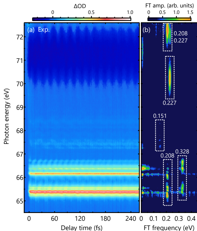
FIG. 2. (a) Experimental delay-dependent transient absorption spectra of DBr. The pump and probe pulses are polarized to a parallel direction. Multiple quantum beats are resolved, showing the electronic and vibrational coherences induced by the strong-field ionization. (b) Fourier transformation (FT) of the experimental spectra along the delay axis. Main FT components are marked by dashed boxes with the numbers indicating the beat frequencies in units of eV.
