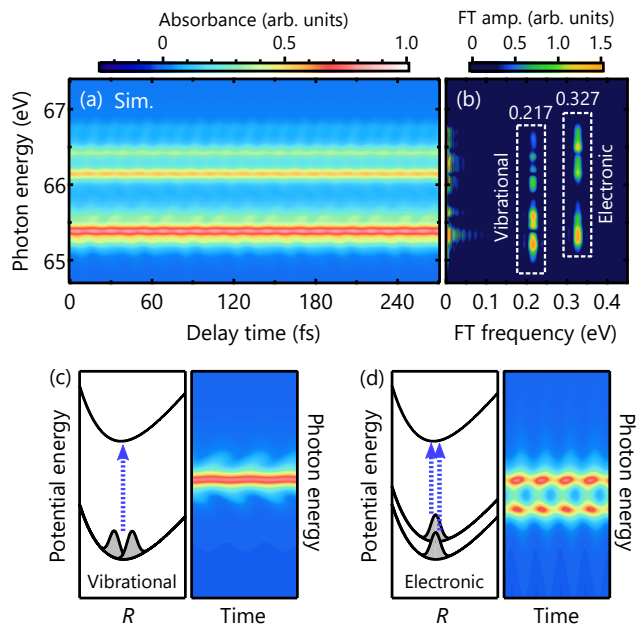
FIG. 3. (a) Simulated delay-dependent transient absorption spectra for the coherent X^2\Pi_{3/2} and X^2\Pi_{1/2} states. (b) Fourier transformation of the simulated spectra along the delay axis. The 0.217 eV (vibrational) and 0.327 eV (electronic) components successfully reproduce the experimental quantum beats. (c,d) Illustration of the probing mechanisms of vibrational and electronic coherences.
