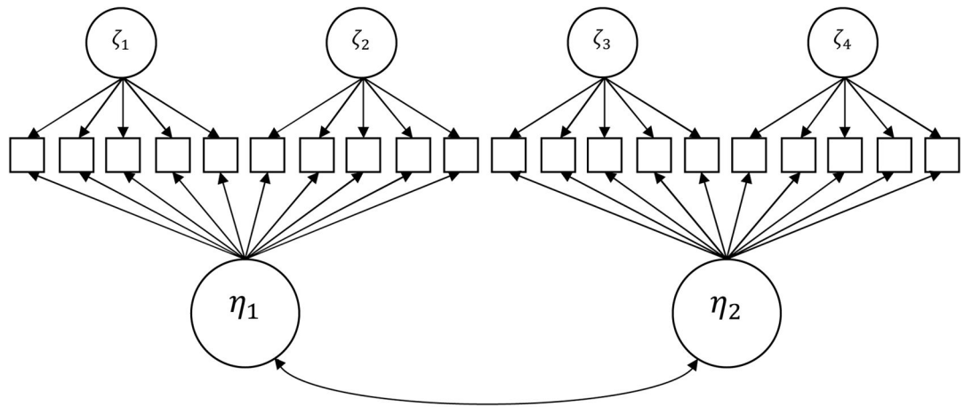
Figure 1. Path diagram of a two-tier model with 2 correlated primary dimensions and 4 specific dimensions.
