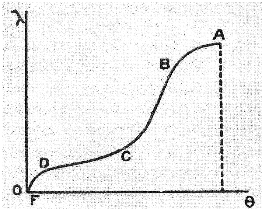
Figure 2: Schematic variation of capillary conductivity \lambda with water content \theta (Buckingham, 1907, Figure 14).
