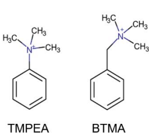
Figure 4. (a) Organic A cation trimethylphenylammonium (TMPEA, left) and benzyltrimethylammonium (BTMA, right). (b) Crystal structure of (TMPEA) 2 MnBr 4 ; Mn...Mn distances: 8.64 Å (shortest) and 9.58 Å labeled with blue dashes. (c) Crystal structure of (BTMA) 2 MnBr 4 , redrawn from ref. 41. Mn...Mn distances: 8.97 Å (shortest) and 9.58 Å labelled with blue dashes.
