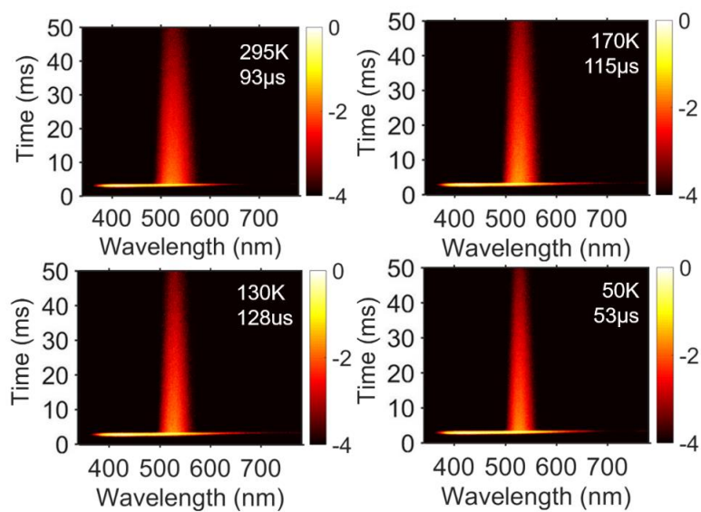
Figure S5. 2D time-resolved PL spectra of (TMPEA) 2 MnBr 4 at selected temperatures. Averaged PL lifetimes are given on the right top corner of each spectrum.
