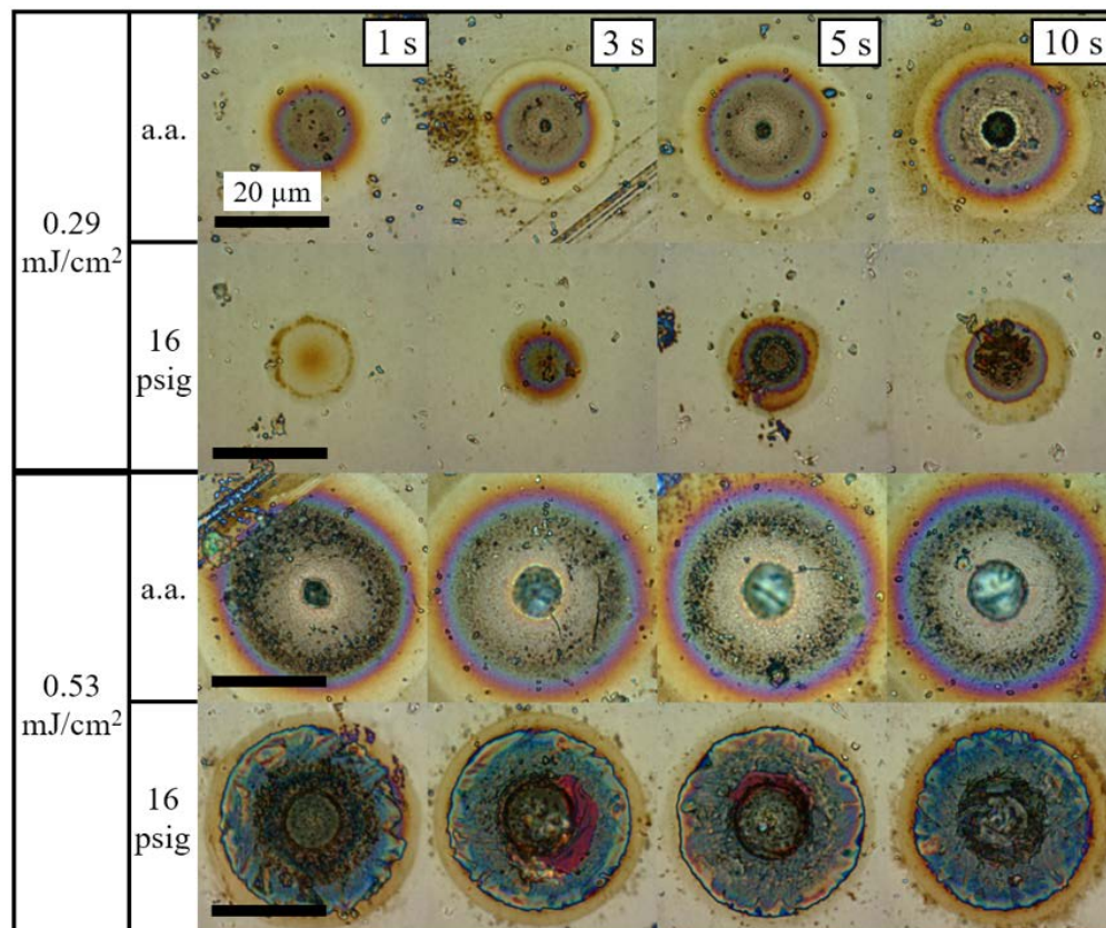
Fig. 4. Light micrographs of molybdenum thin films irradiated for 1, 3, 5 and 10 seconds. Two sets of fluences (0.29 and 0.53 mJ/cm 2 ) and two atmosphere conditions, ambient air (a.a.) and pressurized oxygen at 16 psig are depicted. The scale bar corresponds to 20 \mu\text{m} .
