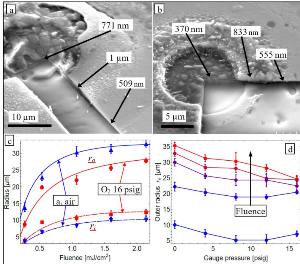
Fig. 7. SEM images of FIB cuts of irradiated molybdenum thin film at ambient air conditions (a) and pressurized oxygen at 8 psig (b). A crater-like morphology is clearly seen as different heights were measured along the cut. c) Inner (dashed line) and outer (solid line) radius as a function of fluence for two different ambient conditions: ambient air (blue symbols) and oxygen at 16 psig (red symbols). Lines are just a guide to the eye. d) Outer radius as a function of gauge pressure for different fluences and 5 s irradiation. In panel d) zero gauge pressure corresponds to ambient air conditions. The top (light red) curve corresponds to the highest fluence ( 2.14 \text{ mJ/cm}^2 ) while the bottom (light blue) curve corresponds to the lowest fluence studied in this work ( 0.29 \text{ mJ/cm}^2 ).
