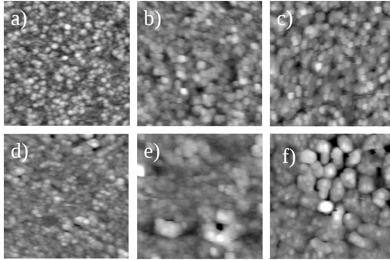
Figure 5. AFM images (2 mm x 2 mm) of the nitrided Ga layers ((a) and (d)), GaN epilayers grown for 5 min on the nitrided Ga layers ((b) and (e)), and GaN epilayers grown for 30 min on the nitrided Ga layers ((c) and (f)). (a), (b), and (c) are for the 5 min Ga metal layer deposition time. (d), (e), and (f) are for the 10 min Ga metal layer deposition time.
