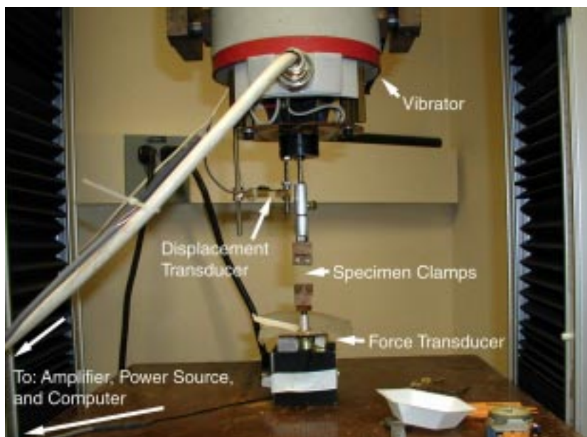
Instrumentation used to test the mechanical properties of egg capsule material. Photos: Scripps Institution of Oceanography
