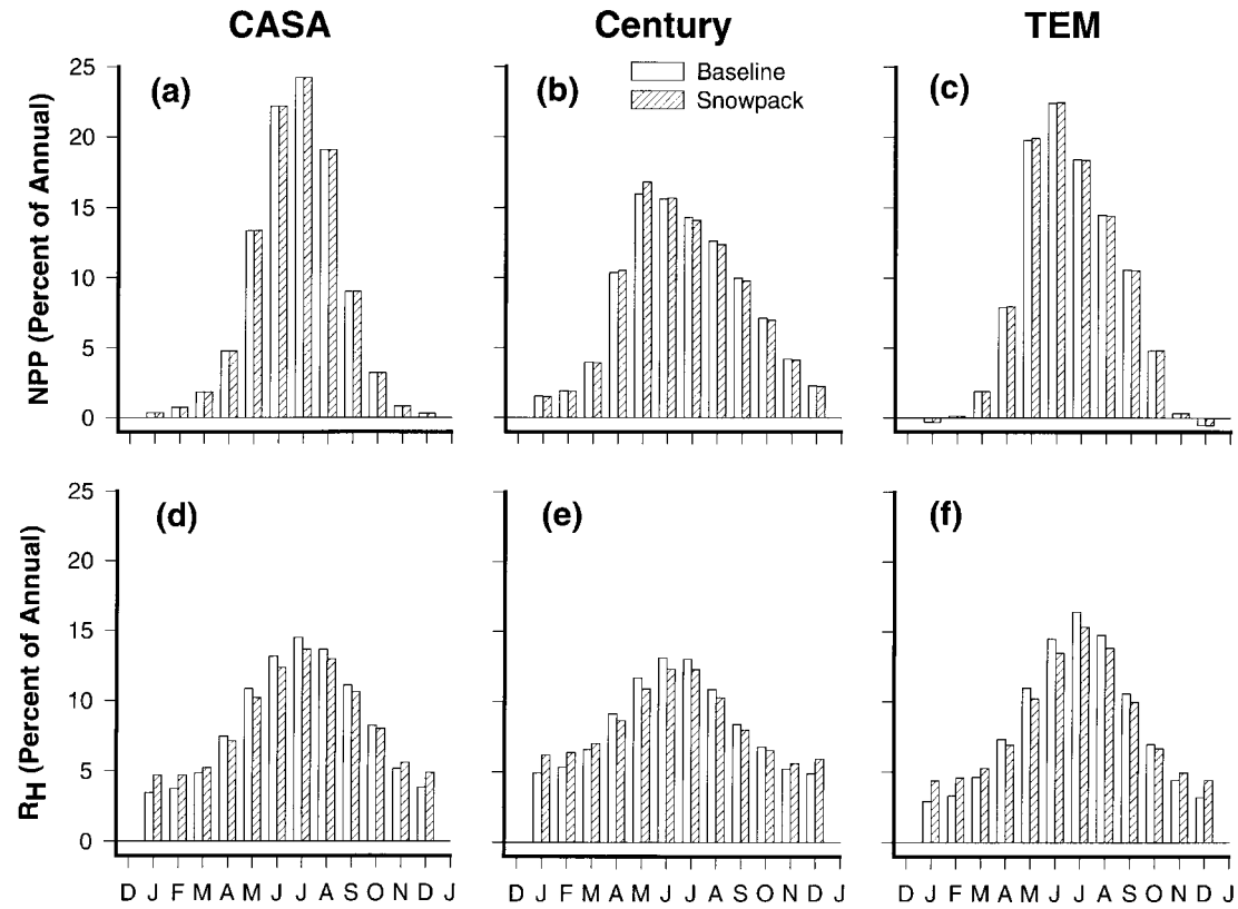
Figure 3. Relative proportions of annual net primary production (NPP) and heterotrophic respiration ( R_H ) that occur during each month of the year for baseline simulations (open bars) and snowpack simulations (hatched bars) between 30^\circ N and 60^\circ N for (a, d) the Carnegie-Ames-Stanford Approach (CASA), (b, e) Century, and (c, f) the Terrestrial Ecosystem Model (TEM).
