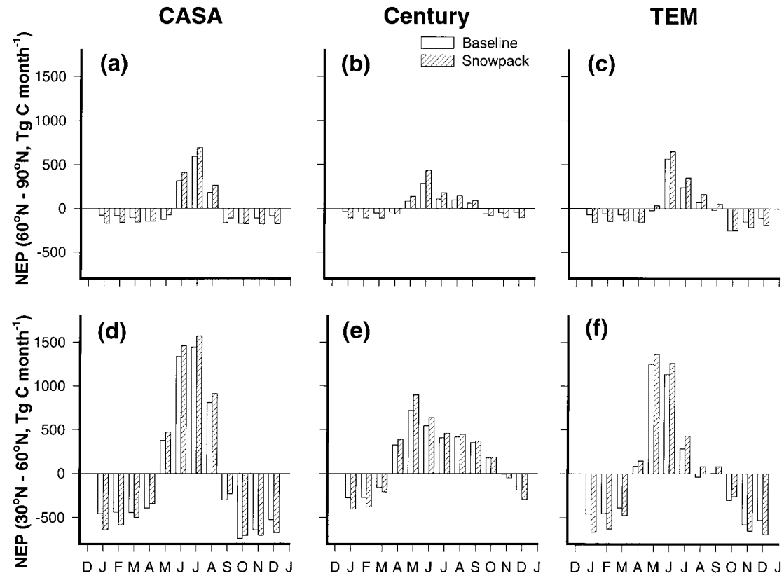
Figure 4. Monthly net ecosystem production (NEP) for baseline simulations (open bars) and snowpack simulations (hatched bars) from (a, b, c) 60° N to 90° N and (d, e, f) 30° N to 60° N for the Carnegie-Ames-Stanford Approach (CASA), Century, and the Terrestrial Ecosystem Model (TEM).
