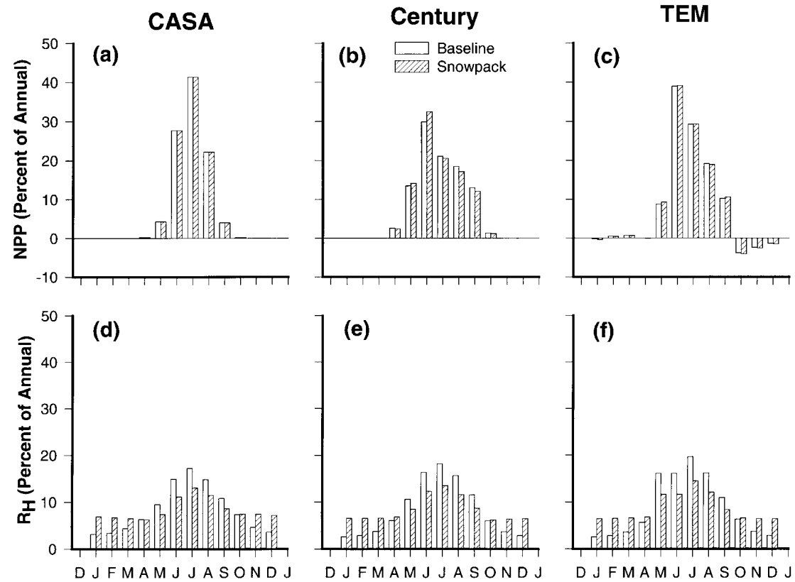
Figure 2. Relative proportions of annual net primary production (NPP) and heterotrophic respiration ( R_H ) that occur during each month of the year for baseline simulations (open bars) and snowpack simulations (hatched bars) between 60^\circ N and 90^\circ N for (a, d) the Carnegie-Ames-Stanford Approach (CASA), (b, e) Century, and (c, f) the Terrestrial Ecosystem Model (TEM).
