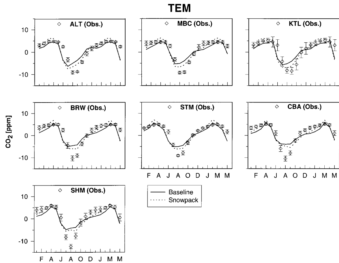
Figure 7. Comparison between the observed seasonal cycle of CO 2 and the simulated seasonal cycle produced by coupling the monthly estimates of net ecosystem production estimated by the Terrestrial Ecosystem Model (TEM) and fossil fuel emissions with the Hamburg ocean and atmospheric transport models for each of the seven high latitude monitoring stations. The first six months of each cycle are displayed twice to reveal the annual variation more clearly. Mean and standard deviation are shown for the observed data. Station abbreviations are identified in Table 1.
