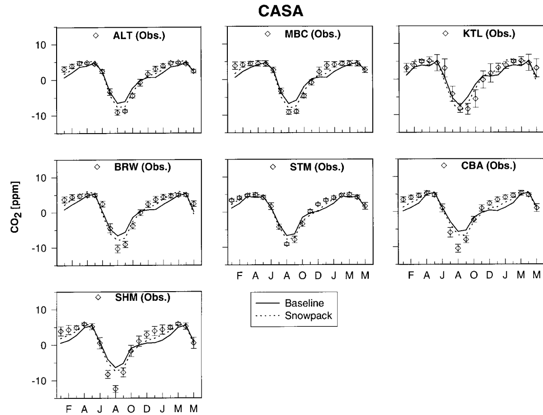
Figure 5. Comparison between the observed seasonal cycle of CO 2 and the simulated seasonal cycle produced by coupling the monthly estimates of net ecosystem production estimated by the Carnegie-Ames-Stanford Approach (CASA) and fossil fuel emissions with the Hamburg ocean and atmospheric transport models for each of the seven high latitude monitoring stations. The first six months of each cycle are displayed twice to reveal the annual variation more clearly. Mean and standard deviation are shown for the observed data. Station abbreviations are identified in Table 1.
