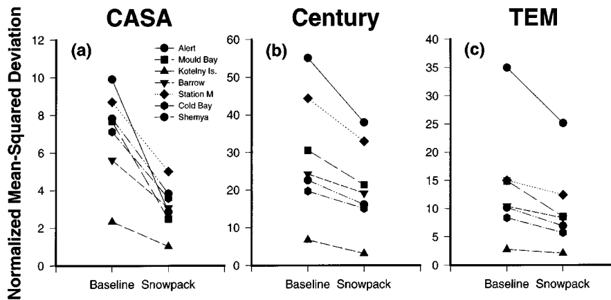
Figure 8. Comparison of the normalized mean-squared deviation between the baseline and snowpack simulations of the seasonal cycle of atmospheric CO 2 at the seven high latitude monitoring stations for (a) the Carnegie-Ames-Stanford Approach (CASA), (b) Century, and (c) the Terrestrial Ecosystem Model (TEM). The normalized mean-squared deviation (nmsd) is an index that indicates the degree of difference between the observed and simulated monthly concentrations of atmospheric CO 2 at a monitoring station, i.e., a nmsd of zero indicates no difference.
