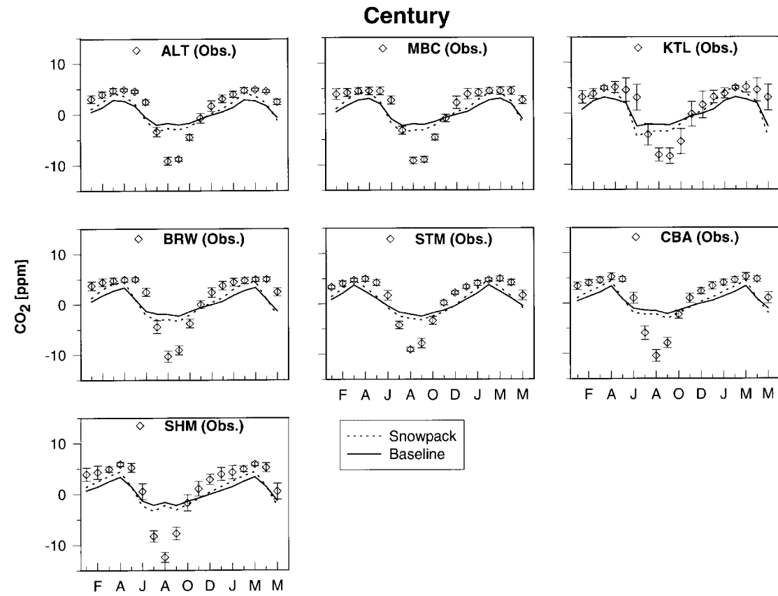
Figure 6. Comparison between the observed seasonal cycle of CO 2 and the simulated seasonal cycle produced by coupling the monthly estimates of net ecosystem production estimated by the Century model and fossil fuel emissions with the Hamburg ocean and atmospheric transport models for each of the seven high latitude monitoring stations. The first six months of each cycle are displayed twice to reveal the annual variation more clearly. Mean and standard deviation are shown for the observed data. Station abbreviations are identified in Table 1.
