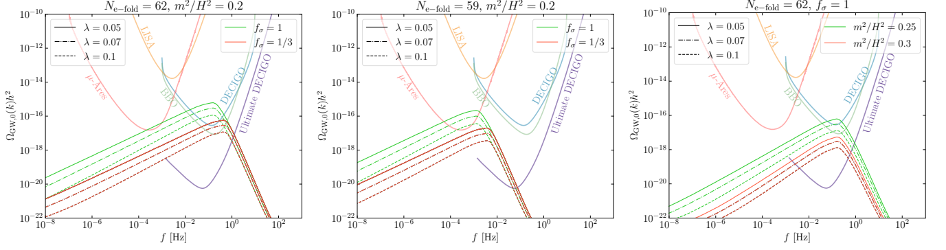
Figure 5. Gravitational wave spectrum for the benchmarks discussed in Fig. 3. We notice that the number of e -folds after CMB-observable modes exited the horizon determines the peak frequency of the spectrum, and correspondingly, different detectors can be sensitive to the signal. Although a similarly peaked spectrum would appear in the context of cosmological phase transitions (PT), the low-frequency tail of this GW spectrum is different from the usual f^3 tail. While in the context of PT the f^3 scaling originates due to causality and superhorizon behavior of fluctuations, in our scenario, the f -scaling is determined by \sigma mass. The differing frequency dependence can then be used to discriminate between the two classes of signals.
