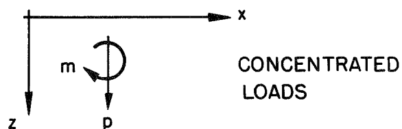
FIGURE III.2 BEAM ELEMENT SIGN CONVENTIONS
