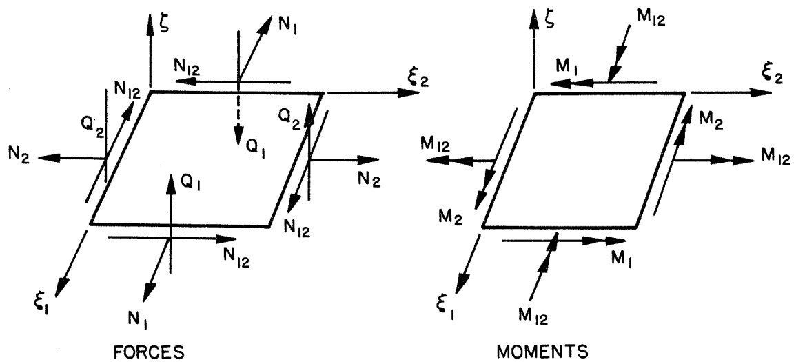
FIGURE II.3 SHELL STRESS RESULTANT SIGN CONVENTIONS
