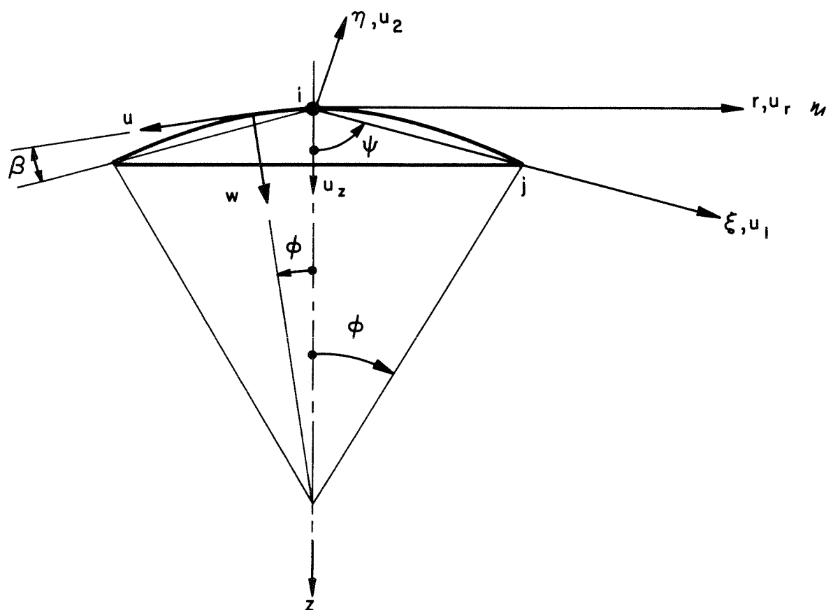
FIGURE III.7 – CAP ELEMENT AFTER KHOJASTEH [84]
