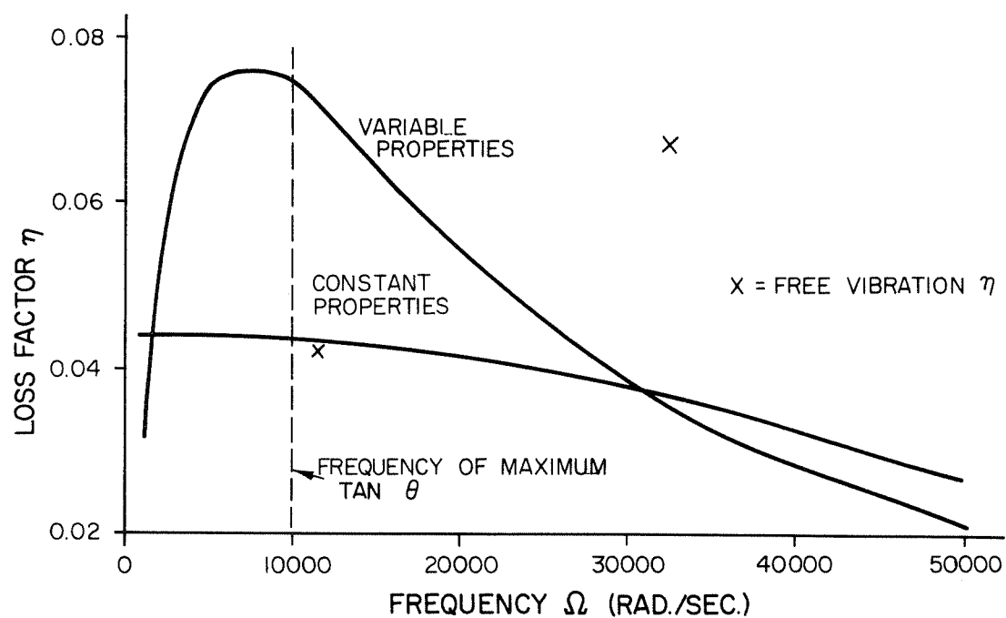
FIGURE V.6 RESPONSE AND DAMPING OF A SANDWICH BEAM FOR LOAD CASE I
