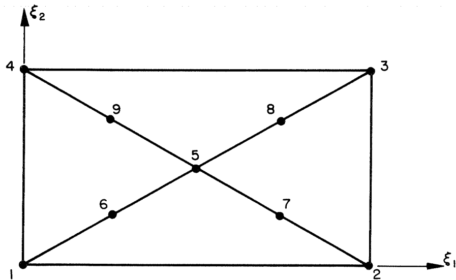
FIGURE II.4 PLANAR QUADRILATERAL ELEMENT AFTER JOHNSON [76]
