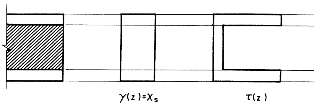
(c) PRESENT APPROXIMATE THEORY - UNWARPED SECTION
