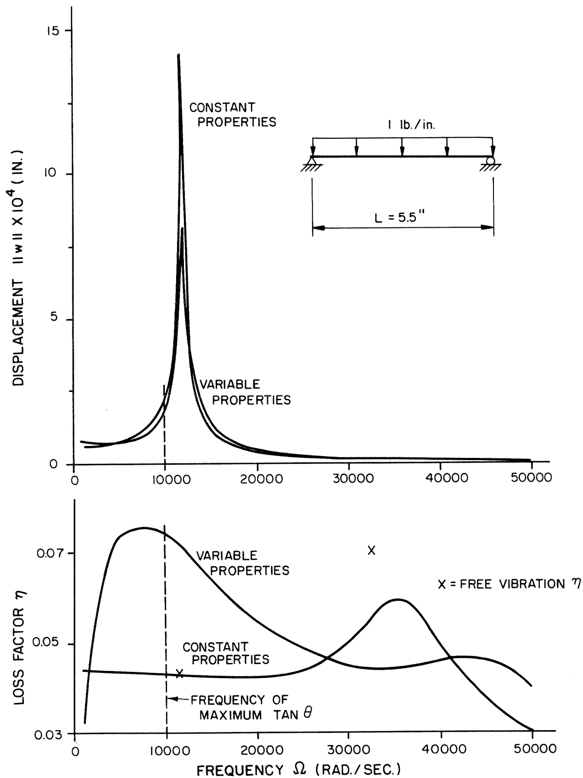
FIGURE V.8 RESPONSE AND DAMPING OF A SANDWICH BEAM FOR LOAD CASE 3
