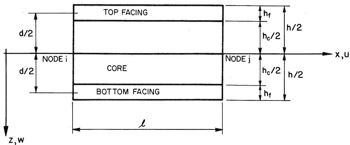
FIGURE III.1 TYPICAL BEAM ELEMENT
