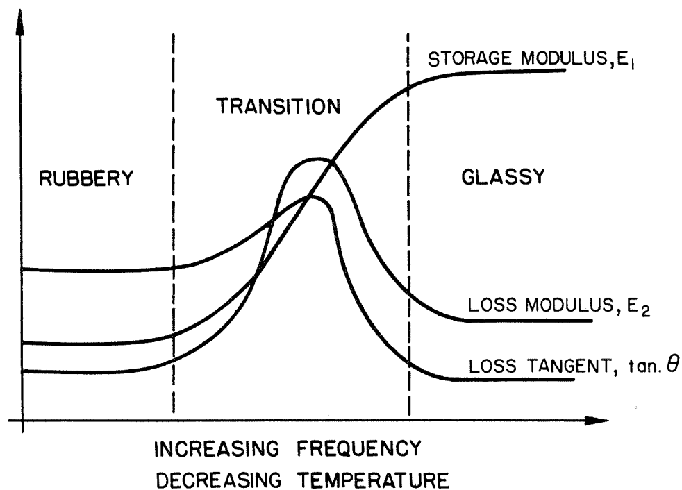
FIGURE V.4 DYNAMIC MECHANICAL DISPERSION
