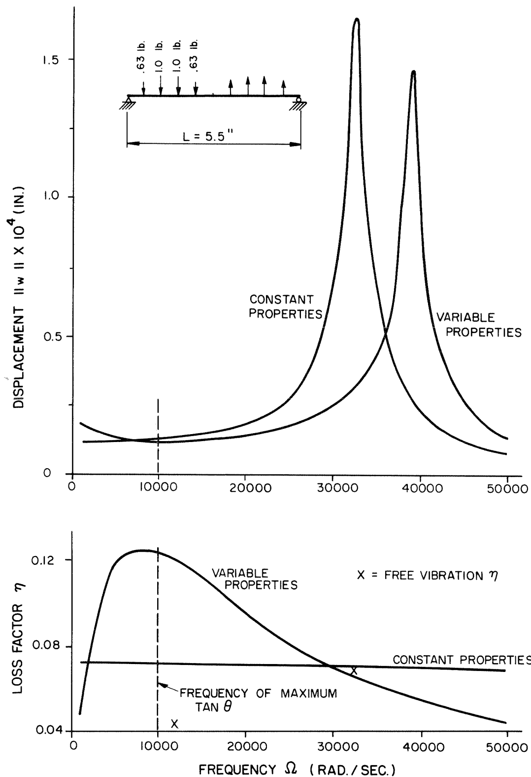
FIGURE V.7 RESPONSE AND DAMPING OF A SANDWICH BEAM FOR LOAD CASE 2
