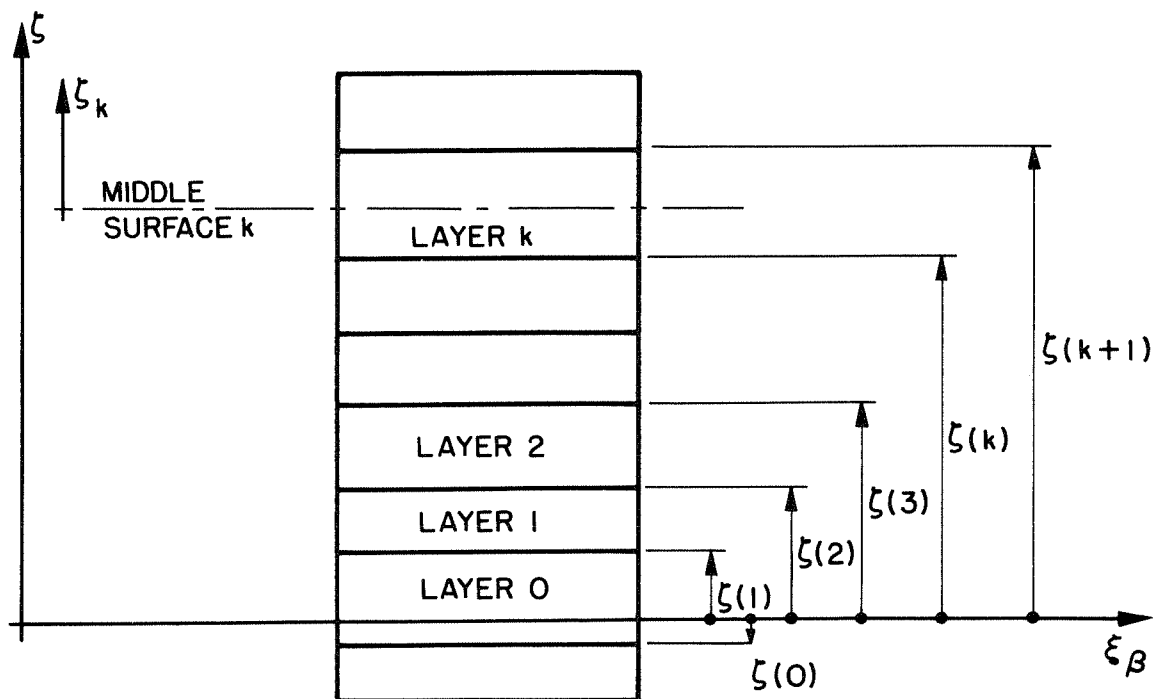
FIGURE II.2 THICKNESS GEOMETRY OF MULTILAYER SHELL
