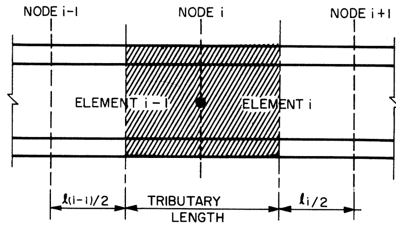
(a) LUMPED MASS FOR TRANSLATIONS
