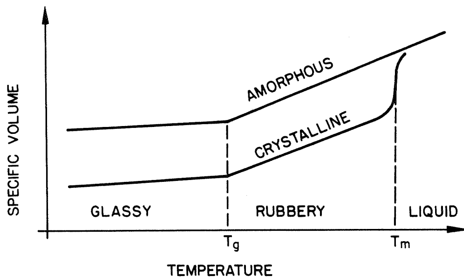
FIGURE V.3 TRANSITION TEMPERATURES OF POLYMERS AFTER NIELSON [140]
