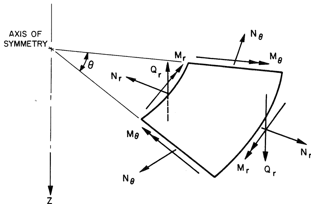
FIG. III.4 AXISYMMETRIC PLATE STRESS RESULTANTS
