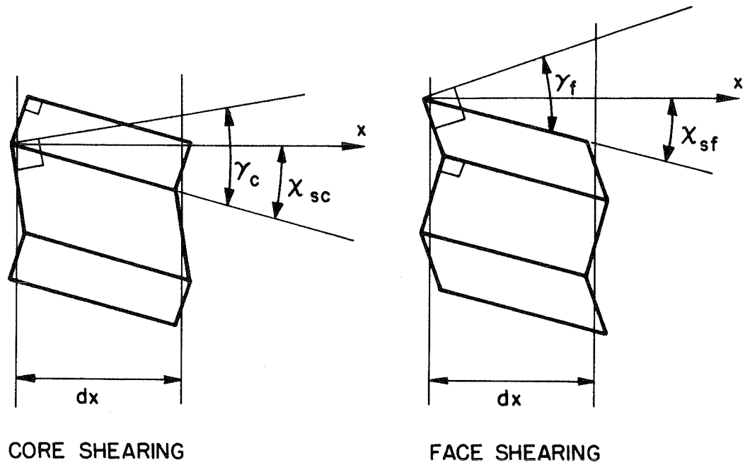
FIGURE III.3 SLOPE DUE TO SHEARING
