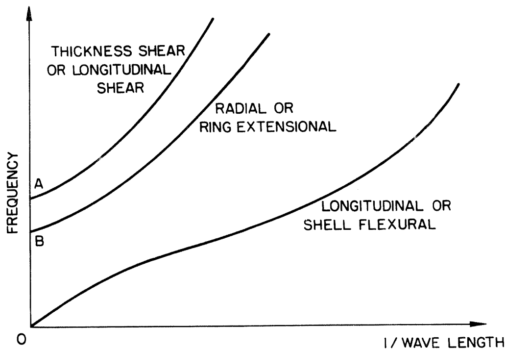
FIGURE IV.3 AXISYMMETRIC VIBRATION MODES OF A CYLINDRICAL SHELL
