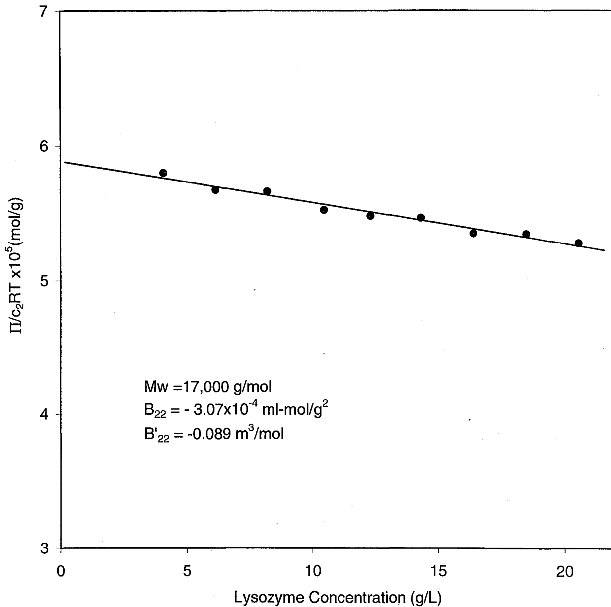
Fig. 2. Osmotic-Pressure Data for Lysozyme at pH 8.0 and 25 °C in 1.0M Ionic Strength (\text{NH}_4)_2\text{SO}_4 Solution.
