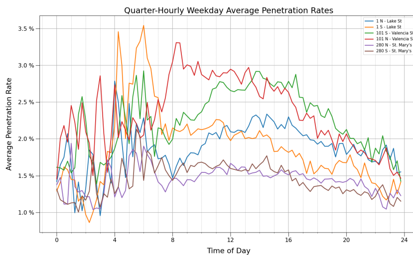
Figure 3.8: Quarter-hourly average penetration rates of SF Highways
