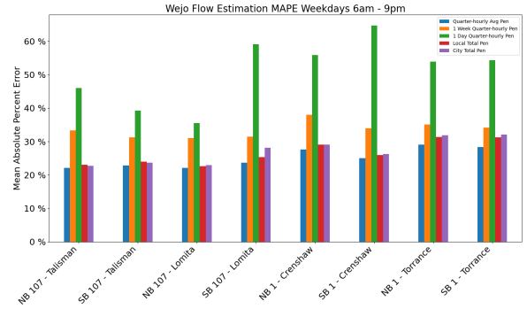
Figure 3.24: LA arterial flow estimation error for different estimates of penetration rate
