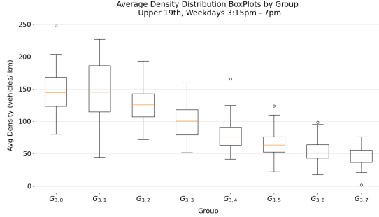
Figure 6.9: Average density of separated 15 minute intervals.
