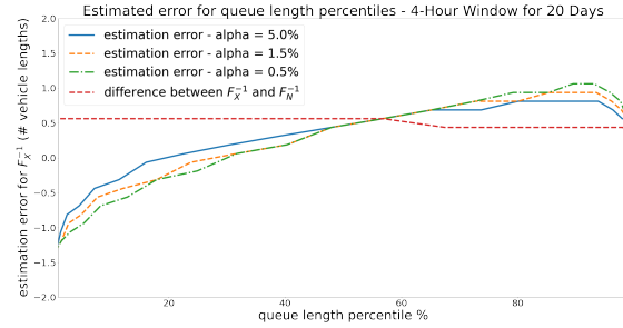
Figure 5.7: Numerical simulation - the estimation error for queue length percentiles F_X^{-1}
