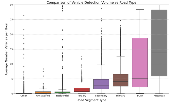
Figure 2.4: Boxplot Distribution of Average Detection Volume in SF by Segment Type
