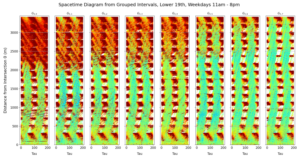
Figure 6.16: Spacetime clusters for lower 19th Avenue 100 second cycletimes
