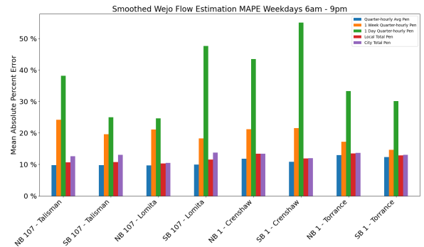
Figure 3.28: Smoothed flow estimation error for LA.
