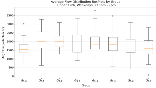
Figure 6.8: Average flow of separated 15 minute intervals.
