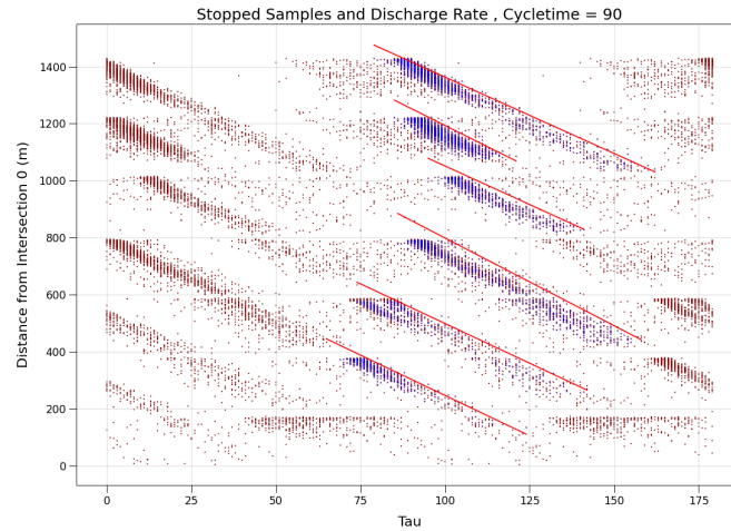
Figure 6.4: Stopped samples of vehicles before moving again along with estimated discharge shockwaves.
