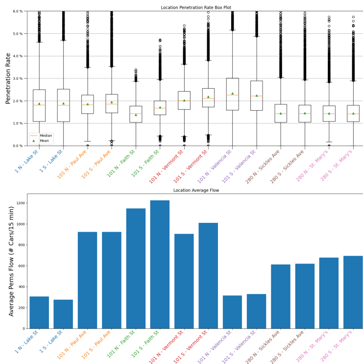
Figure 3.14: Penetration Rate BoxPlots by Location
