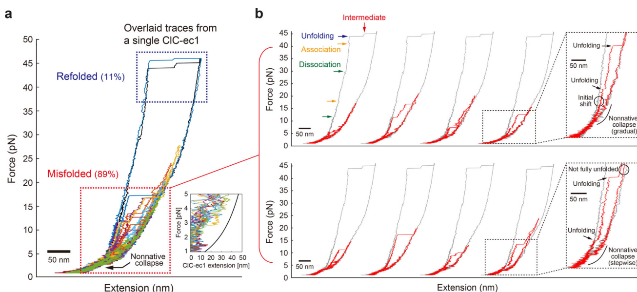
Figure 6. Stable off-pathway misfolded states
