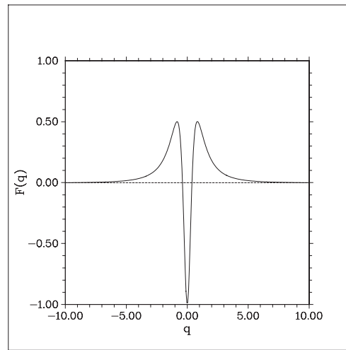
Figure 3: F(q) for the example in Table 1, \Lambda = 1 .
