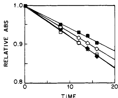
Figure 1. Plots of relative absorbance changes for continuous photolyses of \text{CpFe}(\text{CO})_2(\text{COCH}_3) at 50 and 800 MPa in the presence of \text{P}(\text{OCH}_3)_3 (time is in minutes): filled diamonds, P = 50 MPa, [\text{L}] = 0 ; open squares, P = 800 MPa, [\text{L}] = 0 ; open diamonds, P = 50 MPa, [\text{L}] = 6 \times 10^{-3} M; filled squares, P = 800 MPa, [\text{L}] = 6 \times 10^{-3} M.
