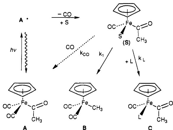
Scheme I. Model for Reactions of the Intermediate S from the Photolysis of CpFe(CO) 2 (COCH 3 ) According to Ref 4 a
