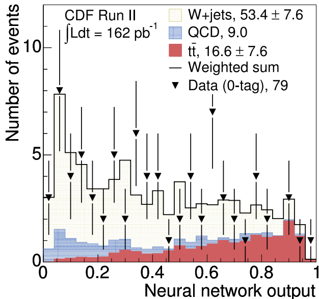
FIG. 1: Fit of the ANN output in the 0-tag L+J data set (triangles) with a sum of 3 components: W +jets (upper), QCD (middle), and t\bar{t} (lower). The QCD normalization is independently estimated and not varied in the fit; its shape is determined from non-isolated lepton data.
