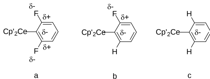
Chart 3: Charge distribution in \text{Cp}'_2\text{CeC}_6\text{H}_{5-x}\text{F}_x
