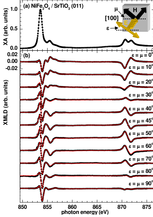
FIG. 1: (Color online) Angular dependence of the Ni L_{2,3} XMLD in NiFe 2 O 4 /SrTiO 3 (011). The inset depicts the experimental geometry. The XMLD spectra are obtained as difference between two XA spectra measured in applied external fields \mathbf{H} (black arrows) at angles \mu and \mu + 90^\circ relative to the [100] axis (dashed line). The x rays impinge on the sample in normal incidence with linear polarization \mathbf{E} (yellow arrow) at an angle \varepsilon to the [100] axis. (a) XA spectrum averaged over all angles \varepsilon . (b) XMLD spectra for \varepsilon = \mu with 0^\circ \leq \mu \leq 90^\circ . Symbols indicate the experimental data and (red) lines give the results of the modeled angular dependence.
