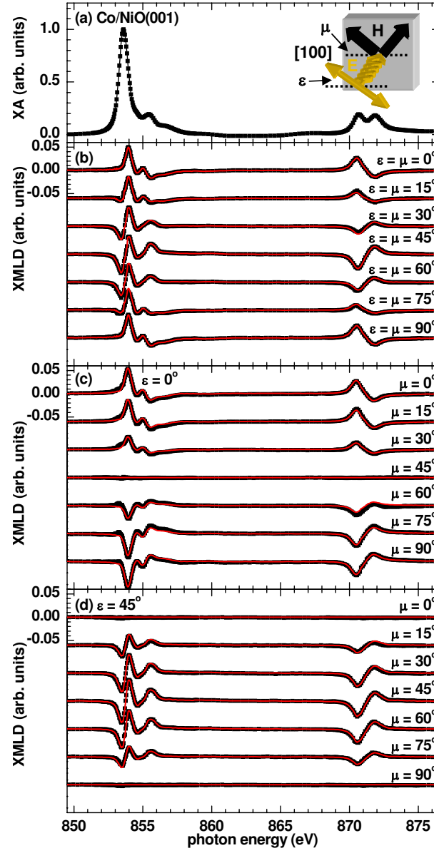
FIG. 3: (Color online) Angular dependence of Ni L_{2,3} XMLD for Co/NiO(001). Solid symbols indicate experimental data while (red) lines show results of the modeled angular dependence. (a) Ni L_{2,3} XA spectrum. The inset shows the experimental geometry as described in Fig. 1(a). XMLD spectra obtained for 0^\circ \leq \mu \leq 90^\circ with (b) \epsilon = \mu , (c) \epsilon = 0^\circ , and (d) \epsilon = 45^\circ .
