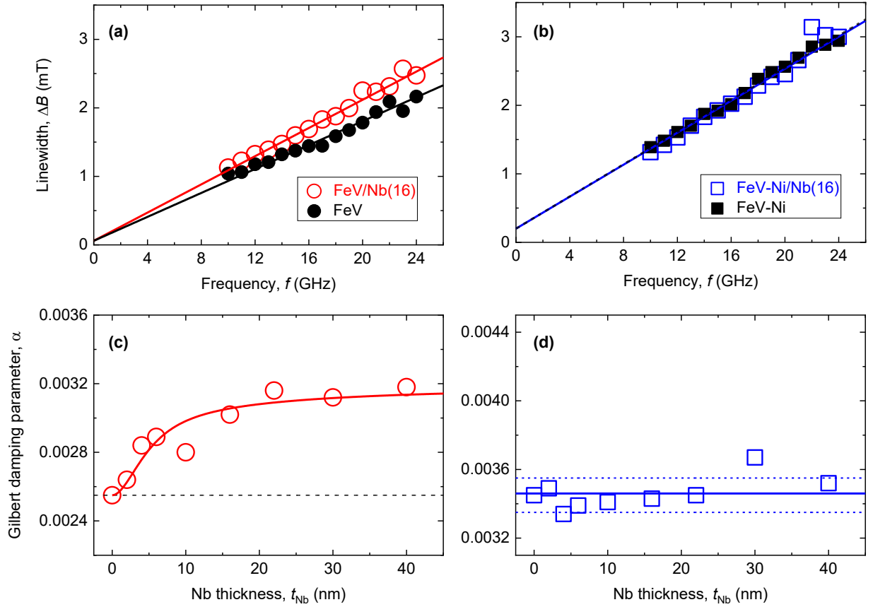
FIG. 3. (a,b) Half-width-at-half-maximum FMR linewidth \Delta B as a function of frequency f for (a) FeV/Nb and (b) FeV-Ni/Nb, measured with the samples magnetized out-of-plane. The linear fits are used to quantify the Gilbert damping parameter \alpha with Eq. 1. (c,d) Gilbert damping parameter \alpha plotted against the Nb thickness for (c) FeV/Nb and (d) FeV-Ni/Nb. The horizontal dashed line in (c) denotes \alpha_{\text{no-sink}} for FeV ( t_{\text{Nb}} = 0 ). In (d), the solid line denotes the average value of \alpha over all FeV-Ni/Nb samples, whereas the dashed lines denote the standard deviation.
