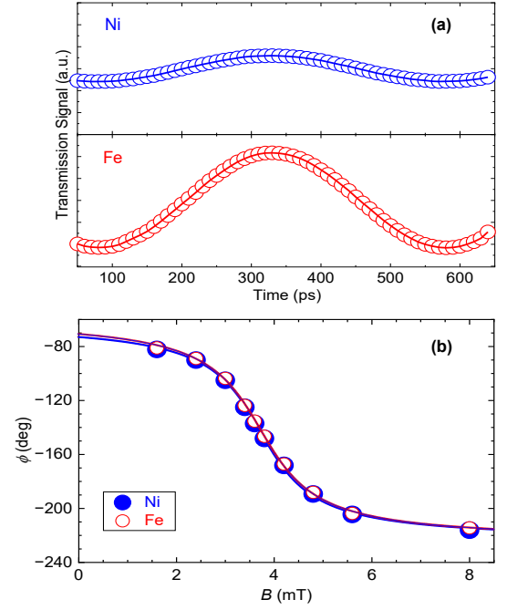
FIG. 2. (a) Time traces of XFMR signals acquired at 2 GHz under an in-plane applied field of 3.7 mT and (b) field dependence of the precessional phase \phi at the Ni and Fe L_3 edges in FeV-Ni ( t_{\text{Nb}} = 0 ).
