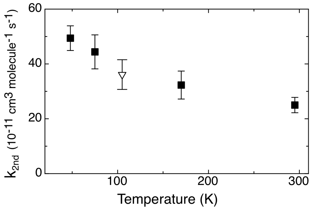
Figure 1. Measured \text{CN} + \text{C}_2\text{H}_4 bimolecular rate coefficient determined in this work at 105 K using ICN as the CN radical photolysis precursor (triangle) compared to the data taken from Sims et al. 17 where NCNO was used as the CN photolysis precursor (squares).
