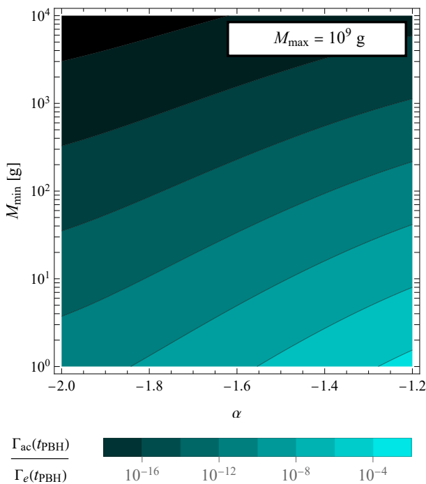
Fig. 6. Contours of \Gamma_{ac}(t_{PBH})/\Gamma_e(t_{PBH}) within the (\alpha, M_{min}) -plane at the beginning of the stasis epoch, where \Gamma_{ac} denotes the total rate of energy-density transfer from radiation to PBHs from accretion and \Gamma_e denotes the total rate of energy-density transfer from PBHs to radiation from evaporation. The results shown correspond to the choice of M_{max} = 10^9 g — a choice which yields the maximum value of this ratio subject to the constraint on M_{max} in Eq. (2.8).
