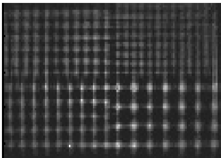
Fig. 7. Simulated sphere sources located at the central plane. The spheres are arranged where the distances between the sources are four times their diameters (like a Derenzo Phantom). The diameters are 1.0 mm, 1.25 mm, 1.5 mm, and 2.0 mm.
