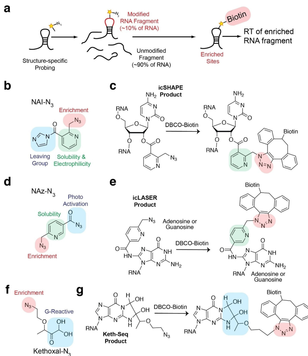
Figure 3. Chemical approaches to enrich modified sites in a complex RNA pool. a) Schematic of chemical probing of RNA structure and enrichment through the use of bi-functional probing reagents. b) Chemical structure of NAI-N 3 , a bi-functional reagent used for icSHAPE probing. c) Chemical structure of biotinylation reaction with NAI-N 3 and DBCO-biotin for biotinylation of icSHAPE adduct sites. d) Chemical structure of NAz-N 3 , a bi-functional reagent used for icLASER probing. e) Chemical structure of biotinylation reaction with NAz-N 3 and with DBCO-biotin for biotinylation of icLASER adduct sites. f) Chemical structure of kethoxal-N 3 , a bi-functional reagent used for icLASER probing. g) Chemical structure of biotinylation reaction with kethoxal-N 3 and DBCO-biotin for biotinylation of keth-seq adduct sites.
