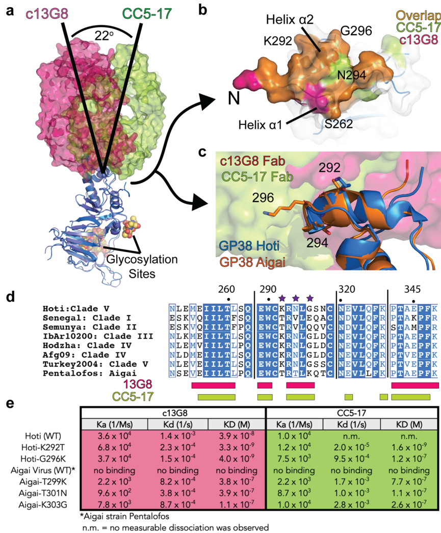
Fig. 3 | GP38 site I investigation. a Comparison of c13G8 (magenta) vs. CC5-17 (lime) engagement with GP38 site I epitope. b Surface area comparison of site I epitope, magenta showing surface area of 13G8 engagement, lime denoting surface area of CC5-17 engagement, and orange denoting the shared surface area of the two Fabs. c Homology model of GP38 from Aigai virus (orange) overlay on complex
