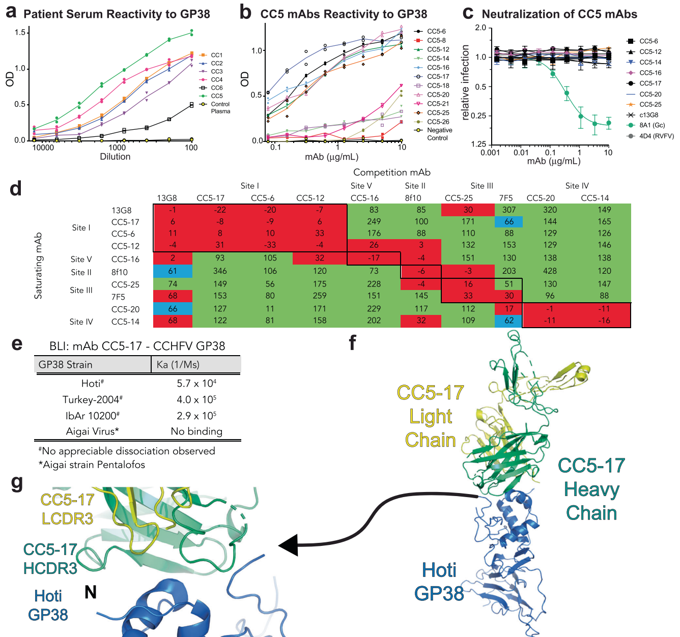
Fig. 2 | Generation of human-derived anti-GP38 mAbs. a Six CCHF survivors in Trabzon (Turkey) were recruited, and their plasma were collected to determine their ELISA titers against GP38 Turkey2004. b Patient CC5 was selected, and its plasma was used to mine 11 mAbs which were then retested against GP38. ELISA experiments were performed in duplicate ( n = 2 ). c Neutralization potential of anti-GP38 mAbs. Foci reduction neutralization assays were performed with CCHFV-ZsG. These data represent one independent experiment out of 2. The average values of replicate wells ( n = 4 ) are plotted, and error bars represent the associated standard
