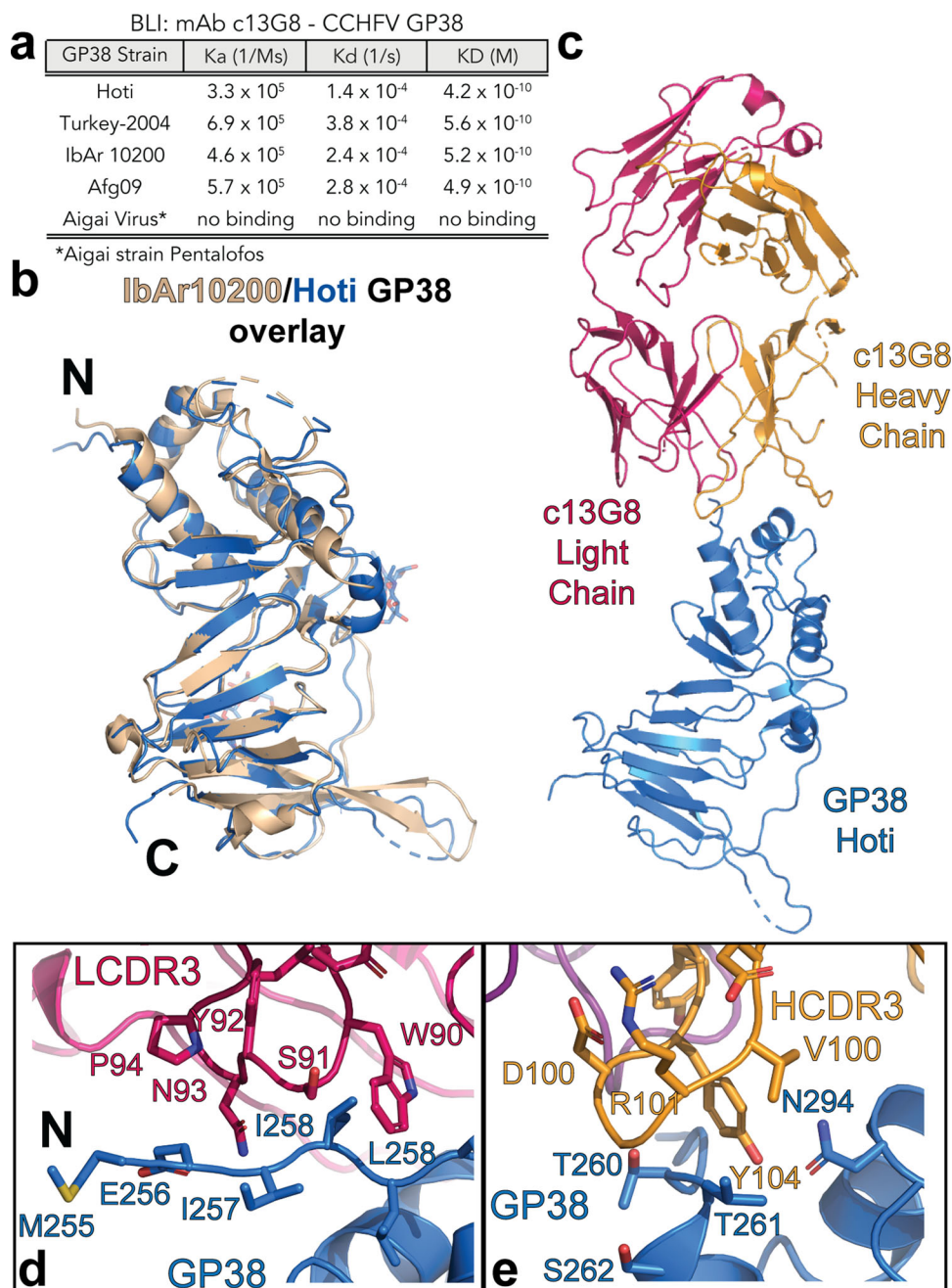
Fig. 1 | c13G8 interactions with nairovirus GP38. a BLI binding kinetics of c13G8 with nairovirus GP38s. b Overlay of CCHFV IbAr10200 GP38 (PDBID 6VKF) (wheat) with our solved CCHFV Hoti GP38 Structure (PDBID 8DC5) (blue) c , c13G8 Fab
