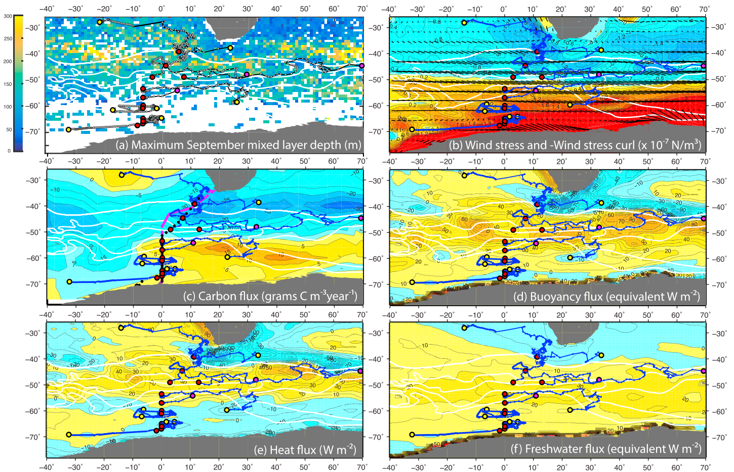
Figure 4. (a) Average maximum September mixed layer depth (m) from all Argo profiles 2000–2016, using density threshold criterion, in each 1° latitude/longitude bin (Holte et al., 2017; http://mixedlayer.ucsd.edu ). White bins have no September profiles. (b) Wind stress (vectors; \text{N/m}^2 ) and negative wind stress curl ( \times 10^{-7} \text{N/m}^3 ) from NCEP reanalysis 1968–1996 (Kalnay et al., 1996). (c) Surface carbon flux (grams \text{C/m}^2\text{yr} ) (Takahashi et al., 2009). Positive is flux out of the ocean (outgassing). (d) Annual mean surface buoyancy flux converted to equivalent heat flux ( \text{W/m}^2 ), summed from (e) annual mean surface heat flux and (f) annual mean freshwater flux converted to equivalent heat flux, all from Large and Yeager (2009), following Ceroveck et al. (2011). Positive values are flux into the ocean, reducing density. In all panels: RV Polarstern PS89 float deployment locations (red), location at end of February 2018 (yellow), or final location (large magenta). Climatological frontal locations (white) from Orsi et al. (1995) (from south to north: SBDY, SACCF, PF, SAF, STF).
