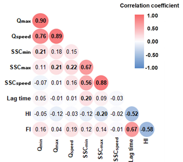
FIGURE 4 Correlations between hysteresis metrics based on all 76 events at the Kings River Experimental Watersheds in the Southern Sierra Nevada, California. Correlation coefficients were estimated using Spearman rank tests and coloured based on their magnitudes and directions. Bolded values were statistically significant ( \alpha = 0.10 )
