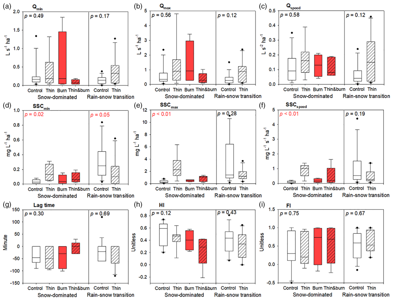
FIGURE 6 Box and whisker plots showing effects of forest thinning and prescribed fire on hysteresis metrics at a higher elevation, snow-dominated site (Bull Creek) and a lower elevation, rain-snow transition site (Providence Creek) at the Kings River Experimental Watersheds in the Southern Sierra Nevada, California. Treatment effects at the snow-dominated site were tested for thin only ( n = 7 ), burn only (4), thin combined with burn (5) and control (12). Treatment effects at the transition site were tested for thin only (11) and control (12); burn only and thin combined with burn were not tested at this site because of limited observations (2 and 1, respectively; Table 2). Data were combined across posttreatment water years (WY 2013–2018). Each boxplot shows the median value (line), interquartile range (box), 90th and 10th percentiles (tails), and outliers falling outside the 90th and 10th percentiles if they occurred (dots). Significance was determined using nonparametric aligned rank transformation tests with repeated measures (indicated with p values in red when statistically significant at \alpha = 0.10 )
