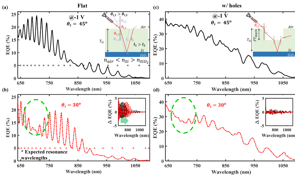
Figure 5. EQE profile as a function of wavelength captured at 45^\circ and 30^\circ angles of incidences of the laser used to illuminate the flat and with-PTMH devices. (a, b) Oscillatory EQE profiles captured for the flat device and the asterisks in (a) and (b), marking the possible resonance wavelengths mathematically calculated for 45^\circ and 30^\circ incidence angles. The inset of (a) shows a schematic of the EM wave refraction while entering the Si region bounded by air and \text{SiO}_2 at two different angles of incidences ( \theta_{i,1} > \theta_{i,2} ) to show path-length modulation ( l_1 > l_2 ). This path-length modulation leads to a systematic shift in the oscillatory \Delta\text{EQE} profile, as shown in the inset of (b). The EQE of the device with-PTMH at (c) 45^\circ and (d) 30^\circ angles of incidences. The presence of PTMH perturbs the smooth resonance process as shown in the inset of (c) and results in the dilution of oscillations and prominent incidence angle dependency as highlighted in the inset of (d). The drop in the EQE near the 700 nm wavelength range in (d) marked with a green dotted line is a residual effect of the prominent drop present near the 700 nm wavelength range in (b) marked with a green dotted line.
