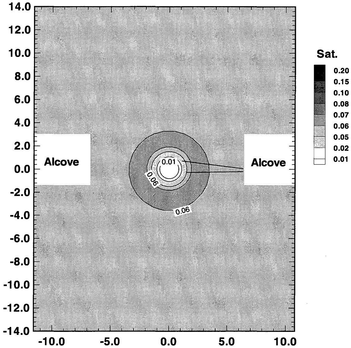
Figure 4.3-2 Fracture liquid saturation for fully homogeneous model domain at 1 year in XZ - cross section at Y = 4.25 m.
